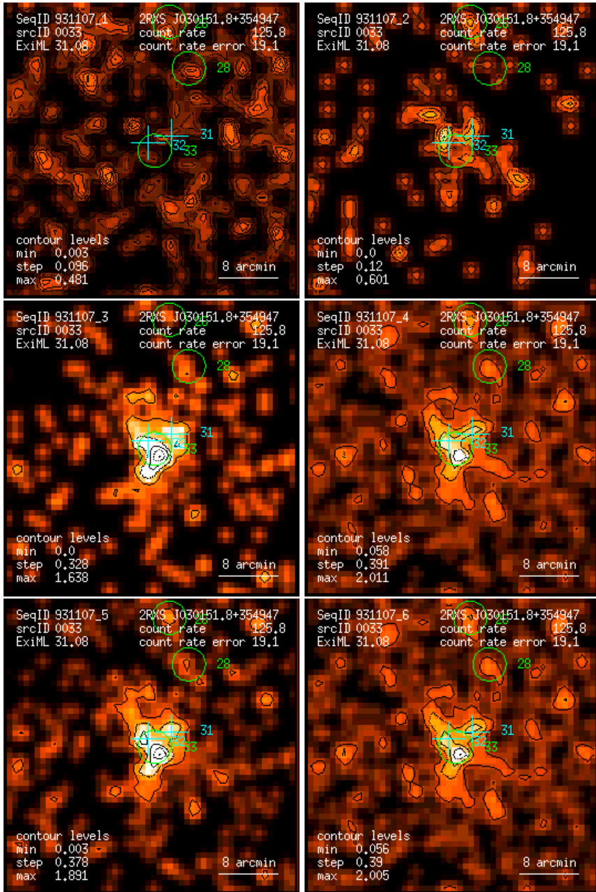
Figure 33: RASS 931107: detection 0033: band rate images, Gaussian filter: (1) PSPC channels 11 – 41, (2) 52 – 90, (3) 91 – 201, (4) 11 – 235, (5) 52 – 201, (6) 11 – 201. Broad band rates in counts/ks. Band rate contour levels in counts/ks/arcmin 2 .
