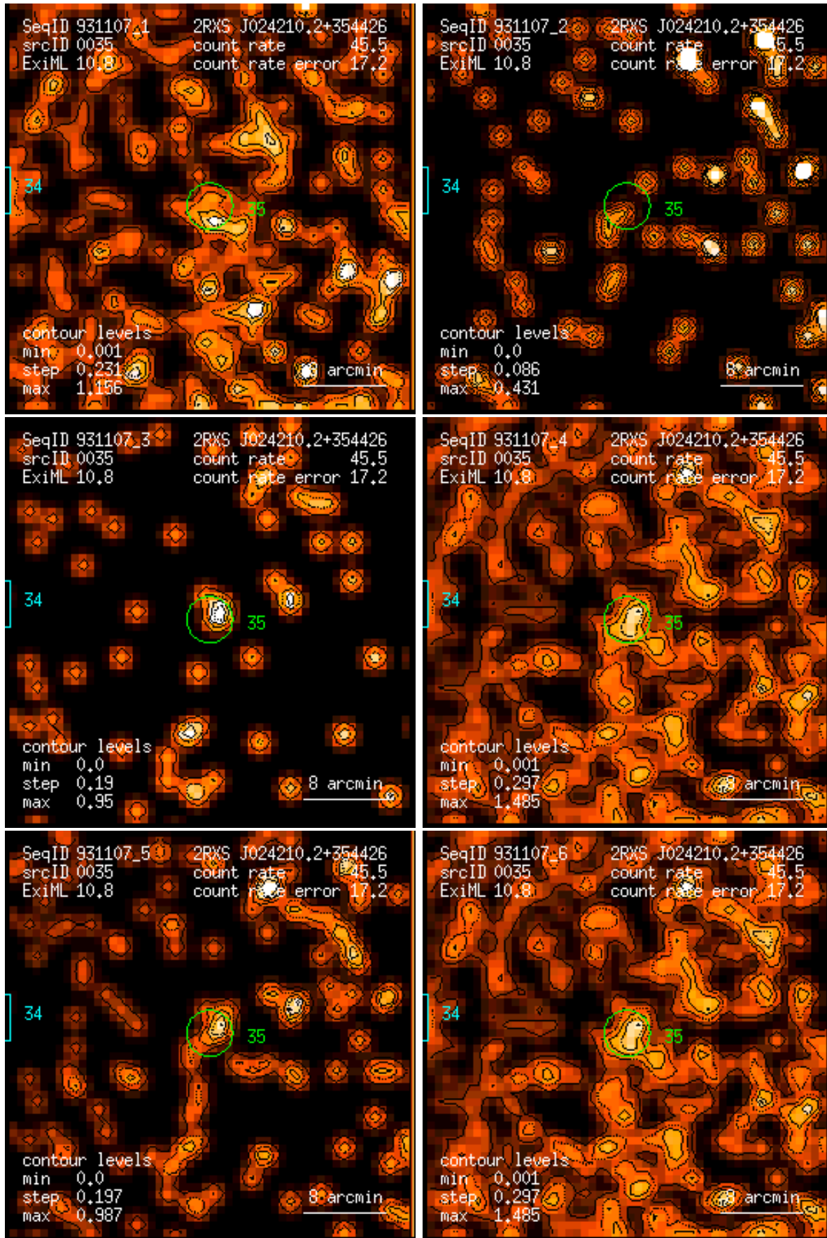
Figure 35: RASS 931107: detection 0035: band rate images, Gaussian filter: (1) PSPC channels 11 – 41, (2) 52 – 90, (3) 91 – 201, (4) 11 – 235, (5) 52 – 201, (6) 11 – 201. Broad band rates in counts/ks. Band rate contour levels in counts/ks/arcmin 2 .
