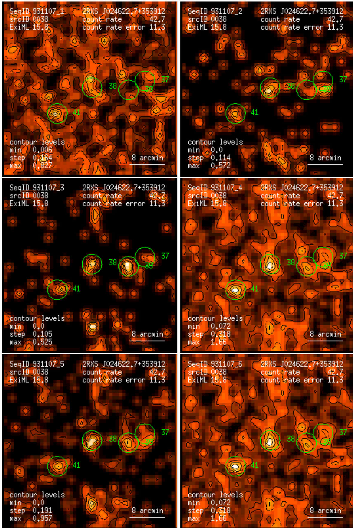
Figure 38: RASS 931107: detection 0038: band rate images, Gaussian filter: (1) PSPC channels 11 – 41, (2) 52 – 90, (3) 91 – 201, (4) 11 – 235, (5) 52 – 201, (6) 11 – 201. Broad band rates in counts/ks. Band rate contour levels in counts/ks/arcmin 2 .
