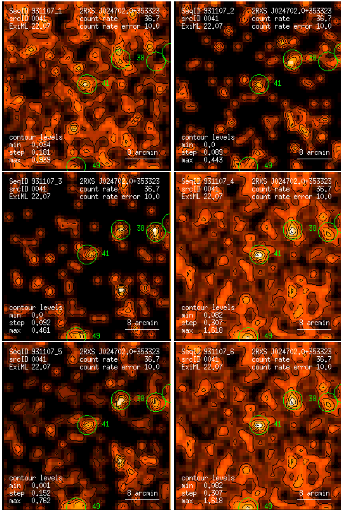
Figure 41: RASS 931107: detection 0041: band rate images, Gaussian filter: (1) PSPC channels 11 – 41, (2) 52 – 90, (3) 91 – 201, (4) 11 – 235, (5) 52 – 201, (6) 11 – 201. Broad band rates in counts/ks. Band rate contour levels in counts/ks/arcmin 2 .
