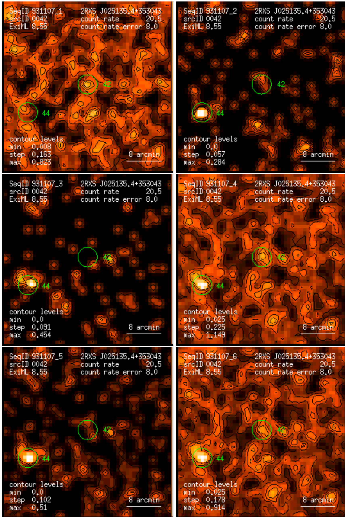
Figure 42: RASS 931107: detection 0042: band rate images, Gaussian filter: (1) PSPC channels 11 – 41, (2) 52 – 90, (3) 91 – 201, (4) 11 – 235, (5) 52 – 201, (6) 11 – 201. Broad band rates in counts/ks. Band rate contour levels in counts/ks/arcmin 2 .
