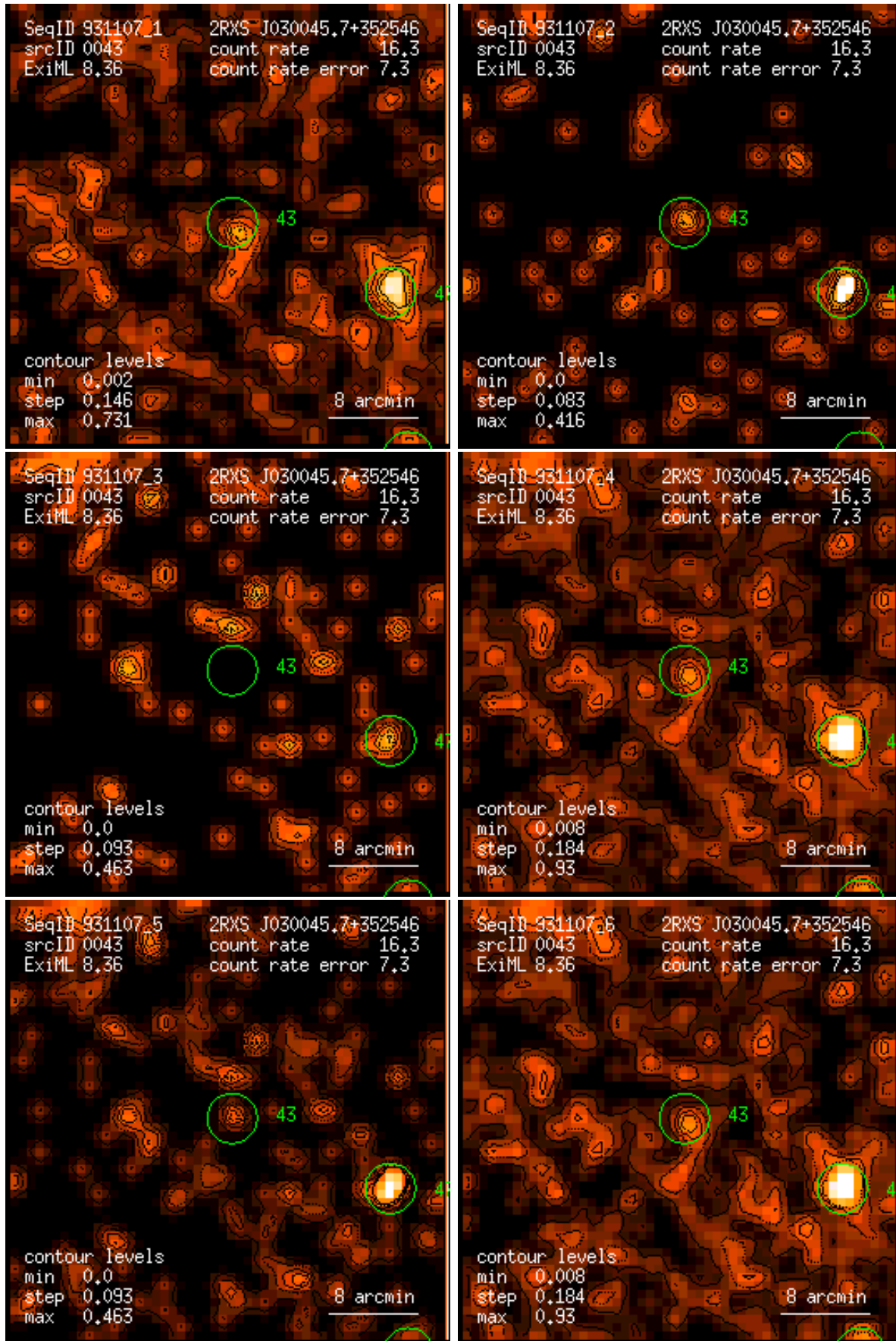
Figure 43: RASS 931107: detection 0043: band rate images, Gaussian filter: (1) PSPC channels 11 – 41, (2) 52 – 90, (3) 91 – 201, (4) 11 – 235, (5) 52 – 201, (6) 11 – 201. Broad band rates in counts/ks. Band rate contour levels in counts/ks/arcmin 2 .
