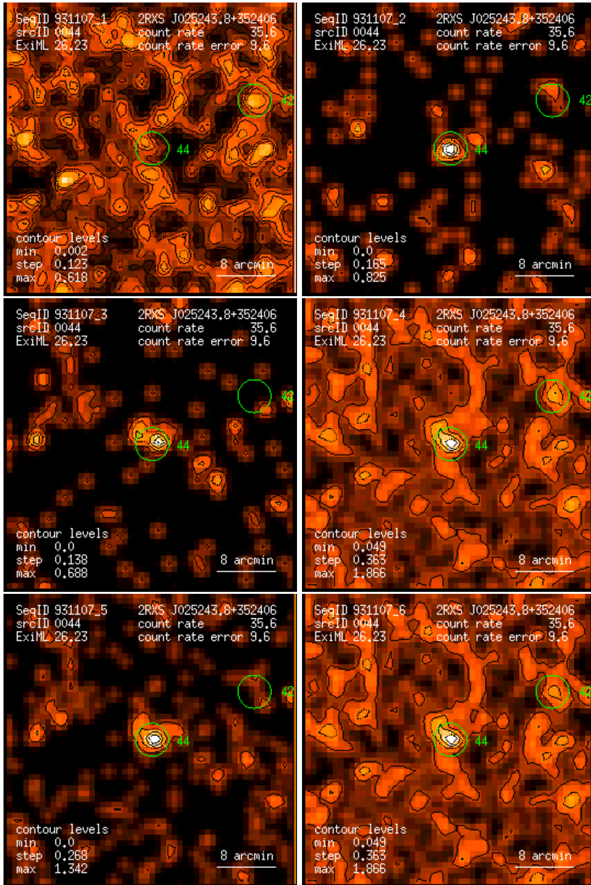
Figure 44: RASS 931107: detection 0044: band rate images, Gaussian filter: (1) PSPC channels 11 – 41, (2) 52 – 90, (3) 91 – 201, (4) 11 – 235, (5) 52 – 201, (6) 11 – 201. Broad band rates in counts/ks. Band rate contour levels in counts/ks/arcmin 2 .
