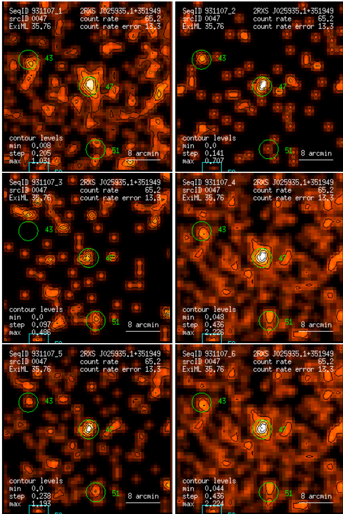
Figure 47: RASS 931107: detection 0047: band rate images, Gaussian filter: (1) PSPC channels 11 – 41, (2) 52 – 90, (3) 91 – 201, (4) 11 – 235, (5) 52 – 201, (6) 11 – 201. Broad band rates in counts/ks. Band rate contour levels in counts/ks/arcmin 2 .
