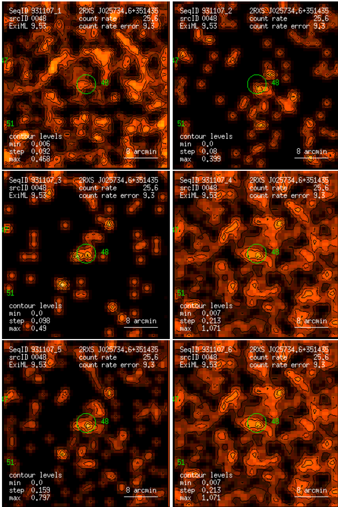
Figure 48: RASS 931107: detection 0048: band rate images, Gaussian filter: (1) PSPC channels 11 – 41, (2) 52 – 90, (3) 91 – 201, (4) 11 – 235, (5) 52 – 201, (6) 11 – 201. Broad band rates in counts/ks. Band rate contour levels in counts/ks/arcmin 2 .
