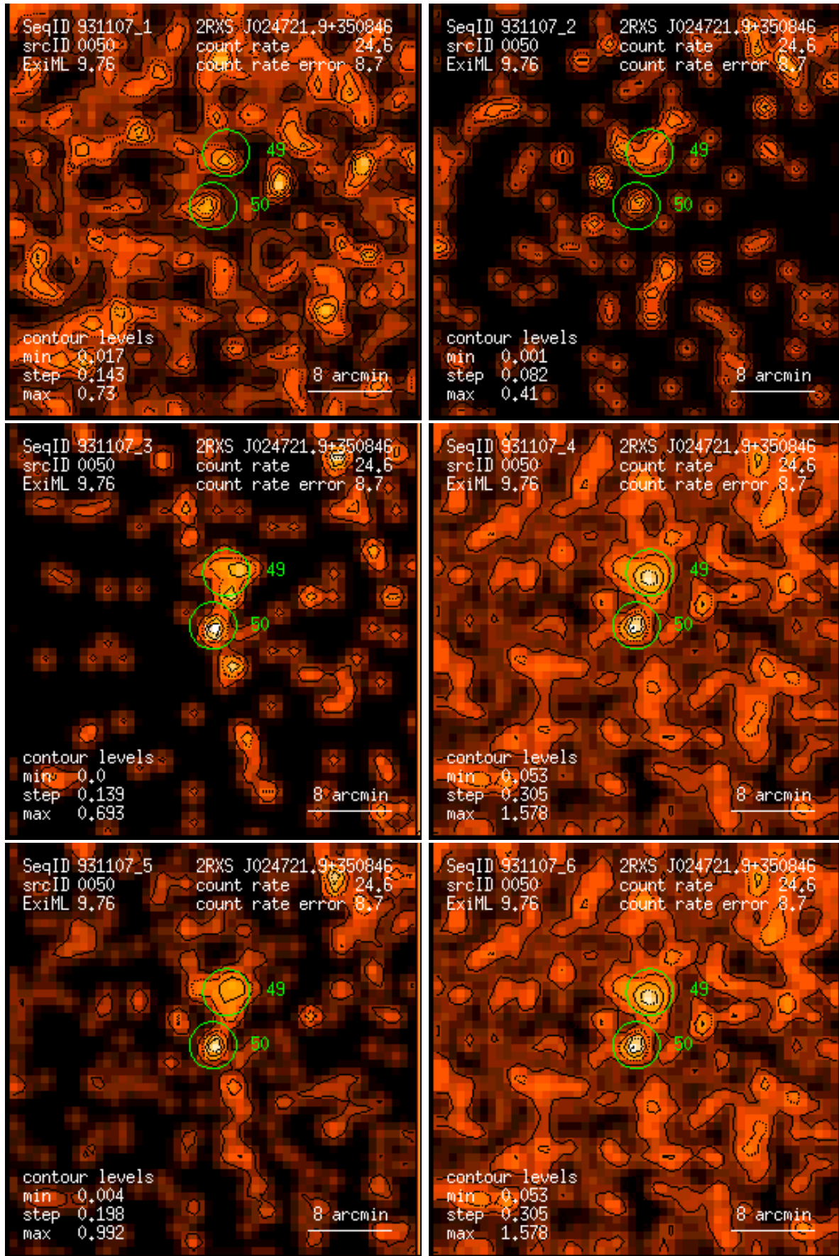
Figure 50: RASS 931107: detection 0050: band rate images, Gaussian filter: (1) PSPC channels 11 – 41, (2) 52 – 90, (3) 91 – 201, (4) 11 – 235, (5) 52 – 201, (6) 11 – 201. Broad band rates in counts/ks. Band rate contour levels in counts/ks/arcmin 2 .
