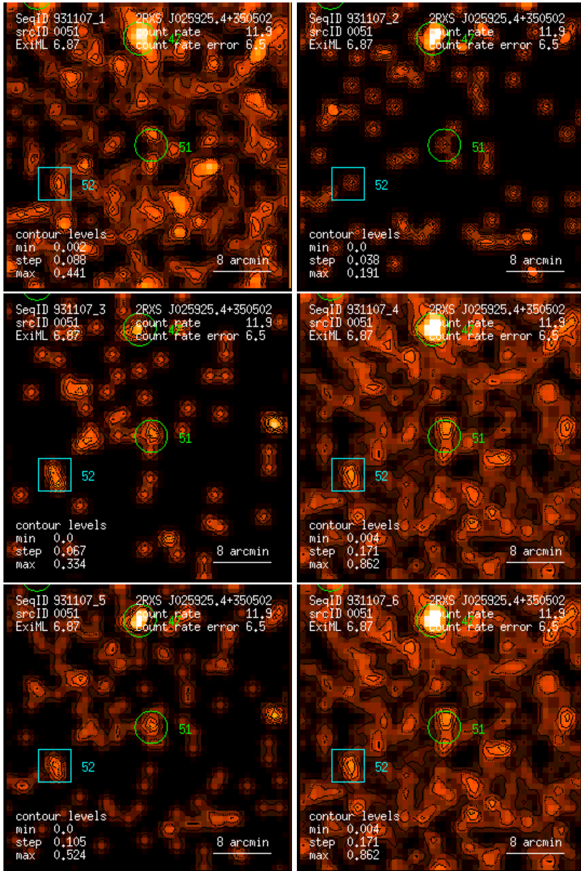
Figure 51: RASS 931107: detection 0051: band rate images, Gaussian filter: (1) PSPC channels 11 – 41, (2) 52 – 90, (3) 91 – 201, (4) 11 – 235, (5) 52 – 201, (6) 11 – 201. Broad band rates in counts/ks. Band rate contour levels in counts/ks/arcmin 2 .
