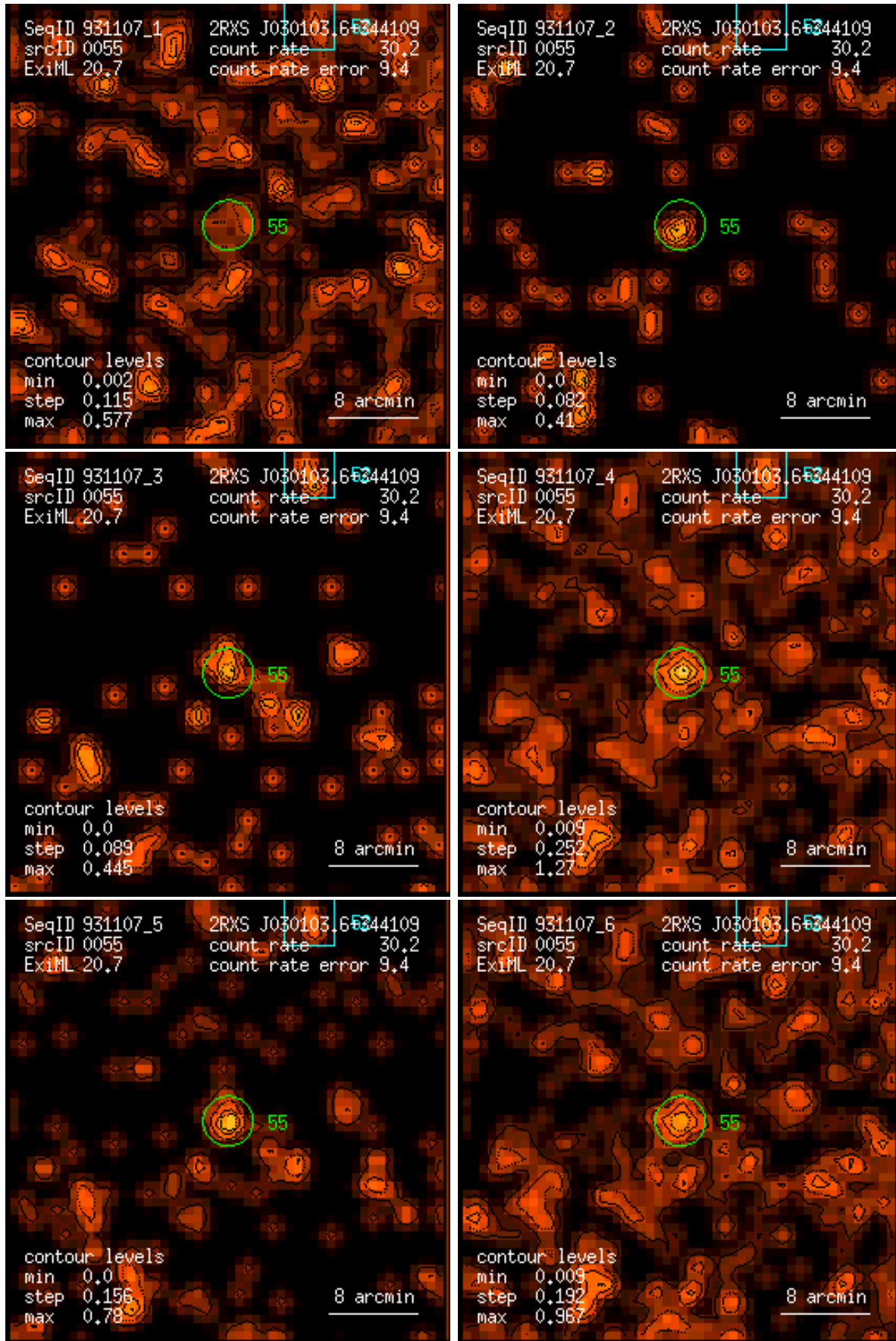
Figure 55: RASS 931107: detection 0055: band rate images, Gaussian filter: (1) PSPC channels 11 – 41, (2) 52 – 90, (3) 91 – 201, (4) 11 – 235, (5) 52 – 201, (6) 11 – 201. Broad band rates in counts/ks. Band rate contour levels in counts/ks/arcmin 2 .
