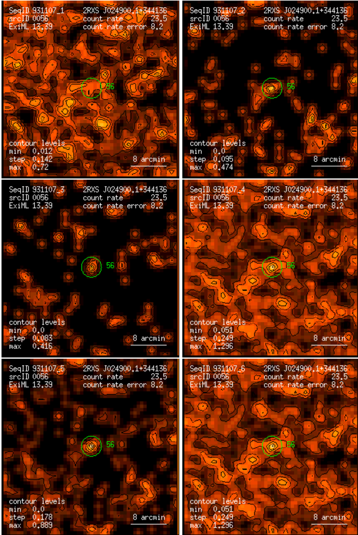
Figure 56: RASS 931107: detection 0056: band rate images, Gaussian filter: (1) PSPC channels 11 – 41, (2) 52 – 90, (3) 91 – 201, (4) 11 – 235, (5) 52 – 201, (6) 11 – 201. Broad band rates in counts/ks. Band rate contour levels in counts/ks/arcmin 2 .
