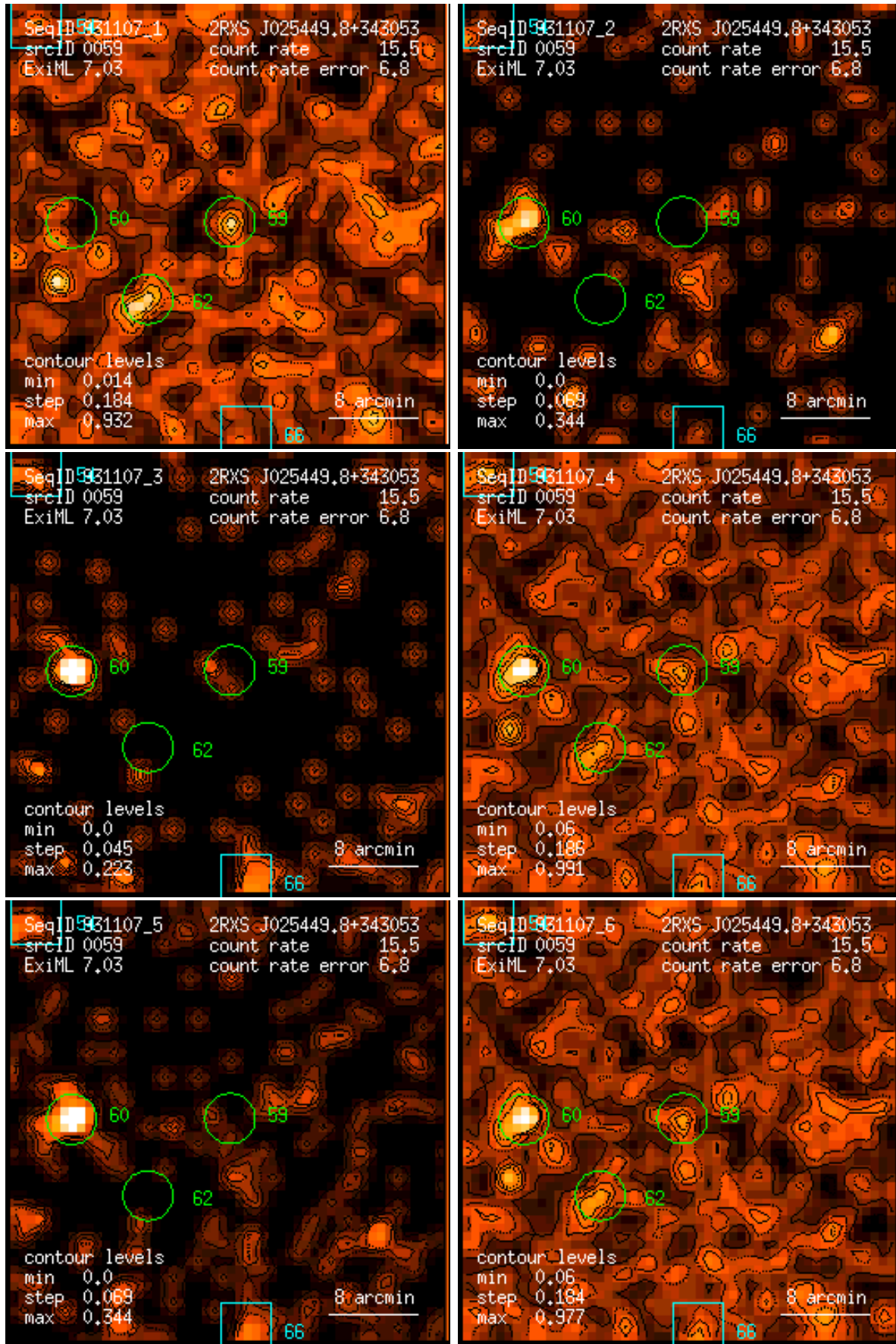
Figure 59: RASS 931107: detection 0059: band rate images, Gaussian filter: (1) PSPC channels 11 – 41, (2) 52 – 90, (3) 91 – 201, (4) 11 – 235, (5) 52 – 201, (6) 11 – 201. Broad band rates in counts/ks. Band rate contour levels in counts/ks/arcmin 2 .
