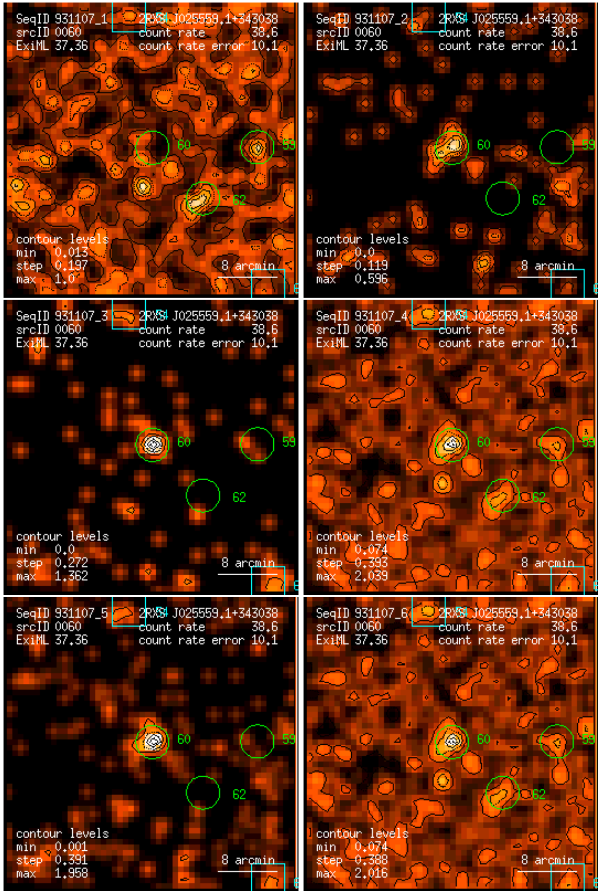
Figure 60: RASS 931107: detection 0060: band rate images, Gaussian filter: (1) PSPC channels 11 – 41, (2) 52 – 90, (3) 91 – 201, (4) 11 – 235, (5) 52 – 201, (6) 11 – 201. Broad band rates in counts/ks. Band rate contour levels in counts/ks/arcmin 2 .
