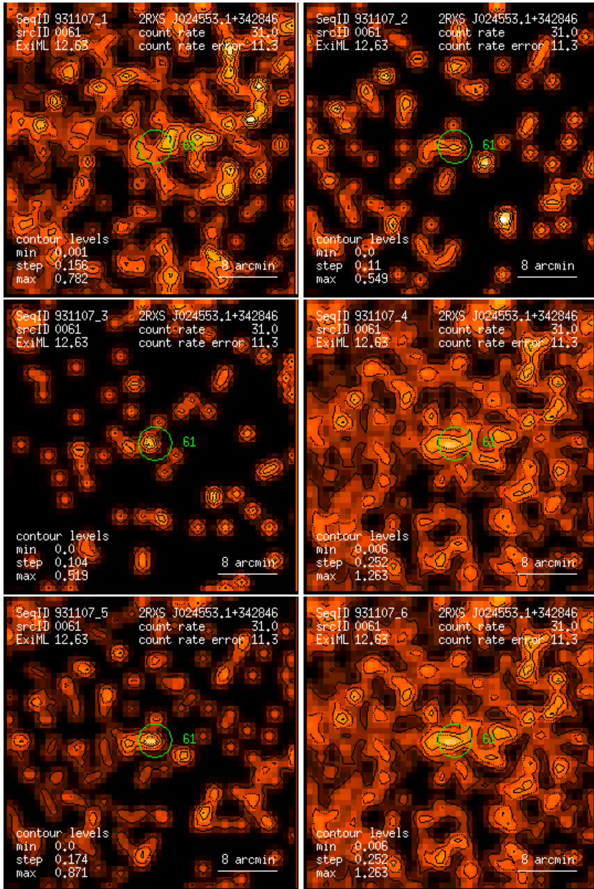
Figure 61: RASS 931107: detection 0061: band rate images, Gaussian filter: (1) PSPC channels 11 – 41, (2) 52 – 90, (3) 91 – 201, (4) 11 – 235, (5) 52 – 201, (6) 11 – 201. Broad band rates in counts/ks. Band rate contour levels in counts/ks/arcmin 2 .
