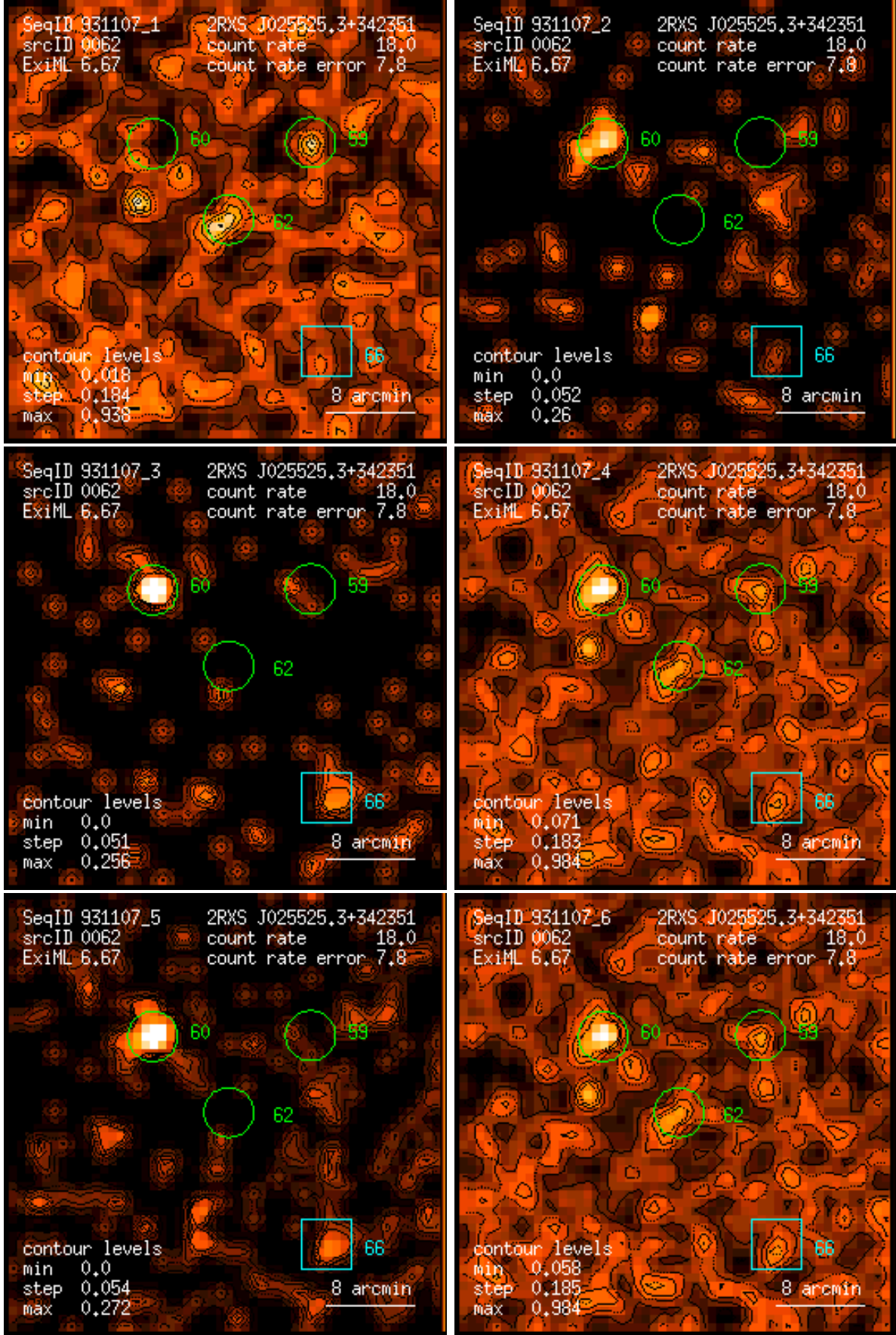
Figure 62: RASS 931107: detection 0062: band rate images, Gaussian filter: (1) PSPC channels 11 – 41, (2) 52 – 90, (3) 91 – 201, (4) 11 – 235, (5) 52 – 201, (6) 11 – 201. Broad band rates in counts/ks. Band rate contour levels in counts/ks/arcmin 2 .
