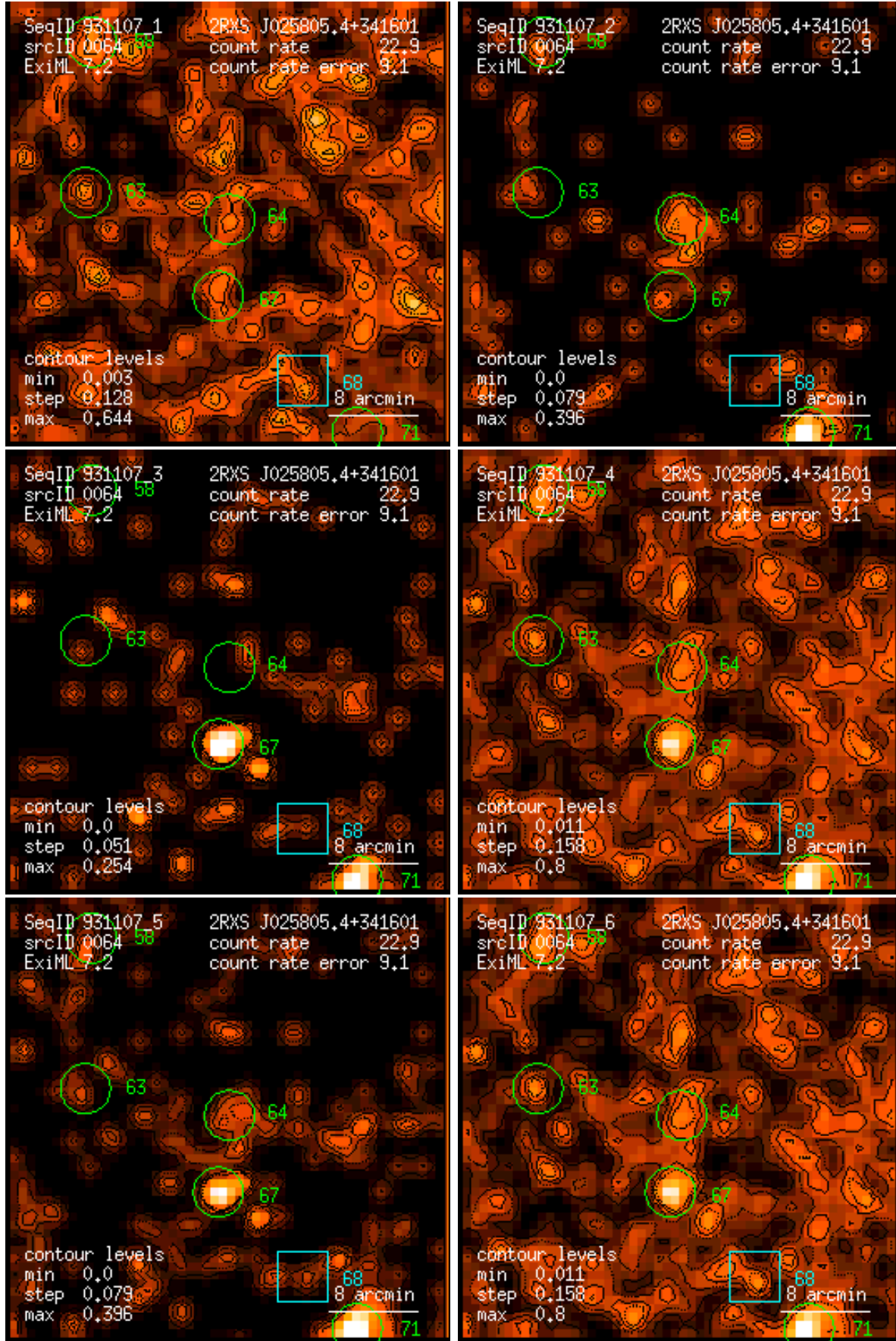
Figure 64: RASS 931107: detection 0064: band rate images, Gaussian filter: (1) PSPC channels 11 – 41, (2) 52 – 90, (3) 91 – 201, (4) 11 – 235, (5) 52 – 201, (6) 11 – 201. Broad band rates in counts/ks. Band rate contour levels in counts/ks/arcmin 2 .
