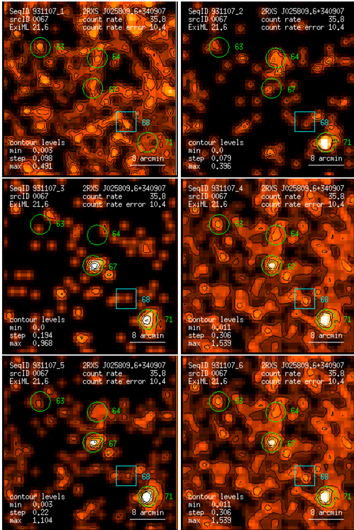
Figure 67: RASS 931107: detection 0067: band rate images, Gaussian filter: (1) PSPC channels 11 – 41, (2) 52 – 90, (3) 91 – 201, (4) 11 – 235, (5) 52 – 201, (6) 11 – 201. Broad band rates in counts/ks. Band rate contour levels in counts/ks/arcmin 2 .
