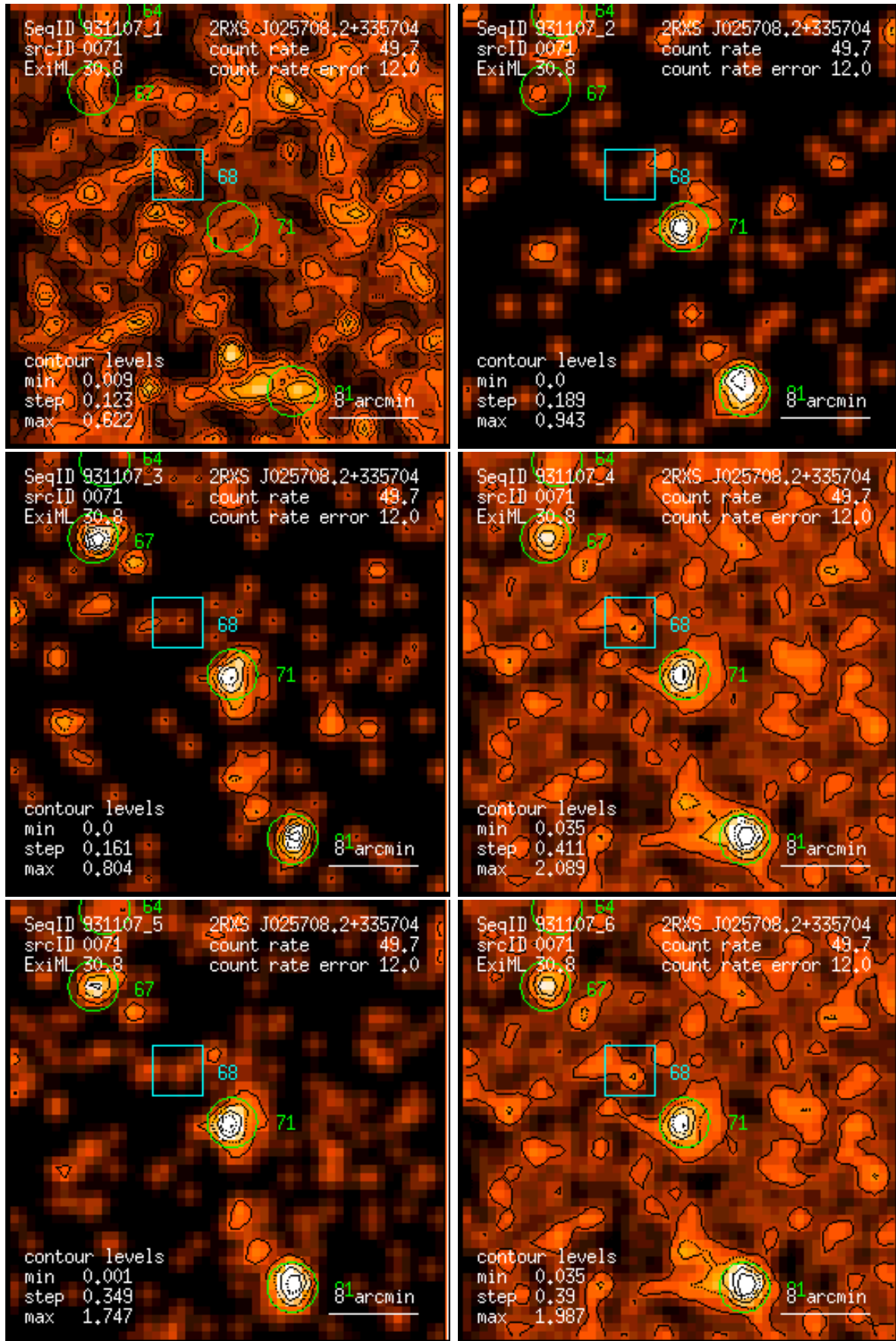
Figure 71: RASS 931107: detection 0071: band rate images, Gaussian filter: (1) PSPC channels 11 – 41, (2) 52 – 90, (3) 91 – 201, (4) 11 – 235, (5) 52 – 201, (6) 11 – 201. Broad band rates in counts/ks. Band rate contour levels in counts/ks/arcmin 2 .
