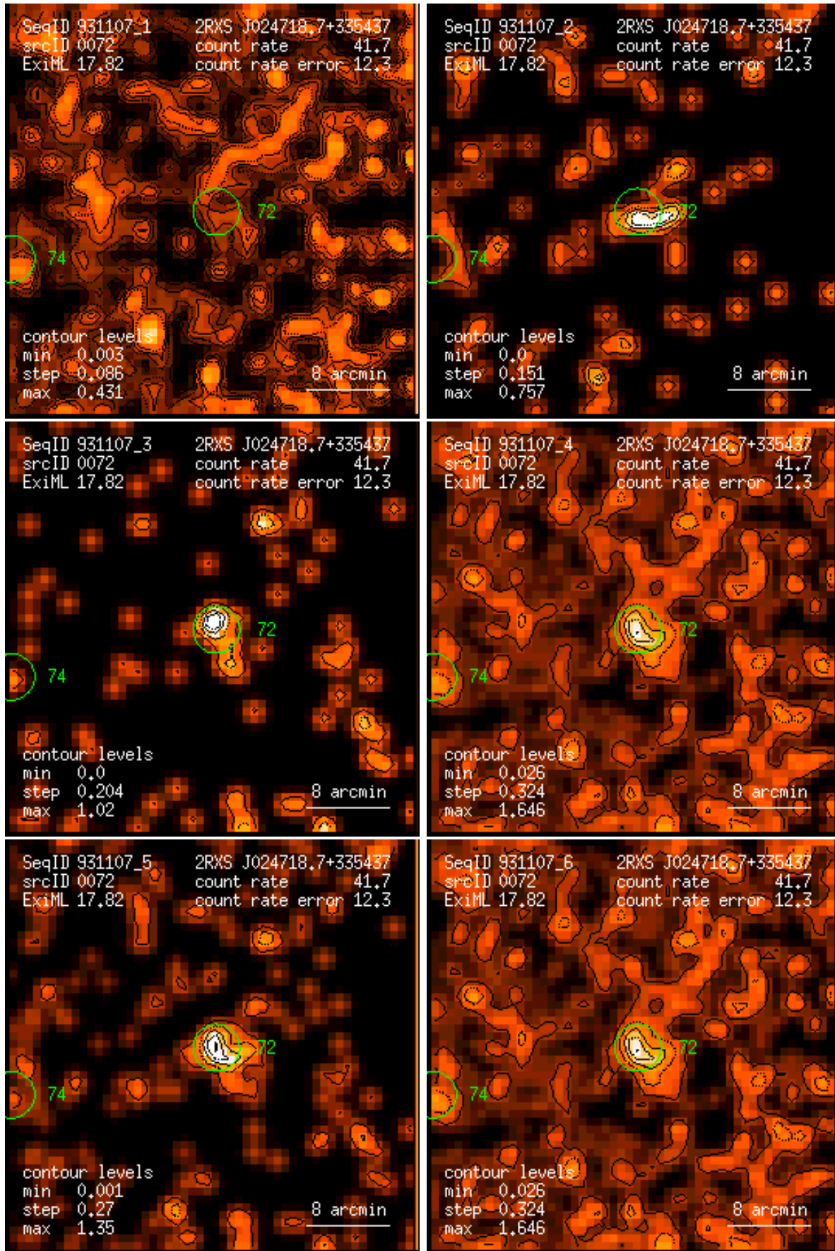
Figure 72: RASS 931107: detection 0072: band rate images, Gaussian filter: (1) PSPC channels 11 – 41, (2) 52 – 90, (3) 91 – 201, (4) 11 – 235, (5) 52 – 201, (6) 11 – 201. Broad band rates in counts/ks. Band rate contour levels in counts/ks/arcmin 2 .
