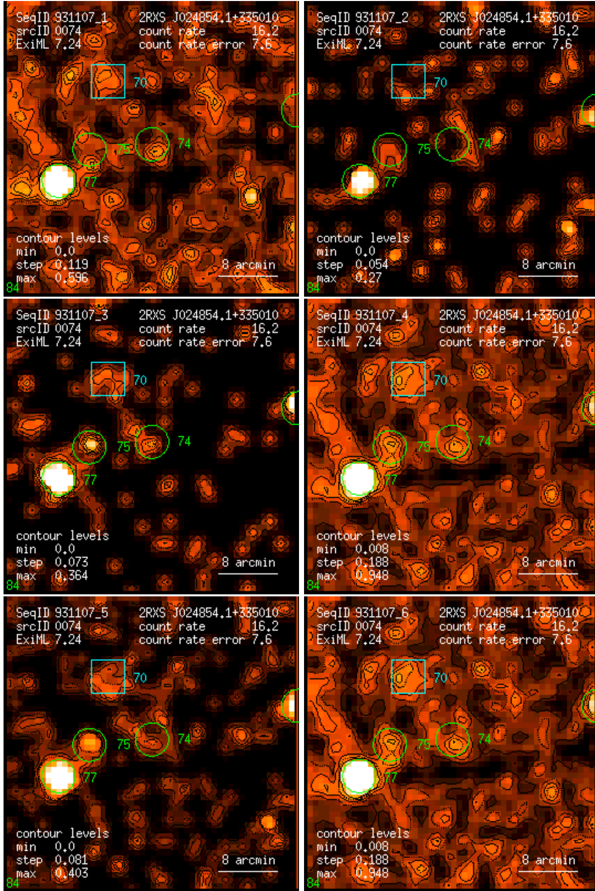
Figure 74: RASS 931107: detection 0074: band rate images, Gaussian filter: (1) PSPC channels 11 – 41, (2) 52 – 90, (3) 91 – 201, (4) 11 – 235, (5) 52 – 201, (6) 11 – 201. Broad band rates in counts/ks. Band rate contour levels in counts/ks/arcmin 2 .
