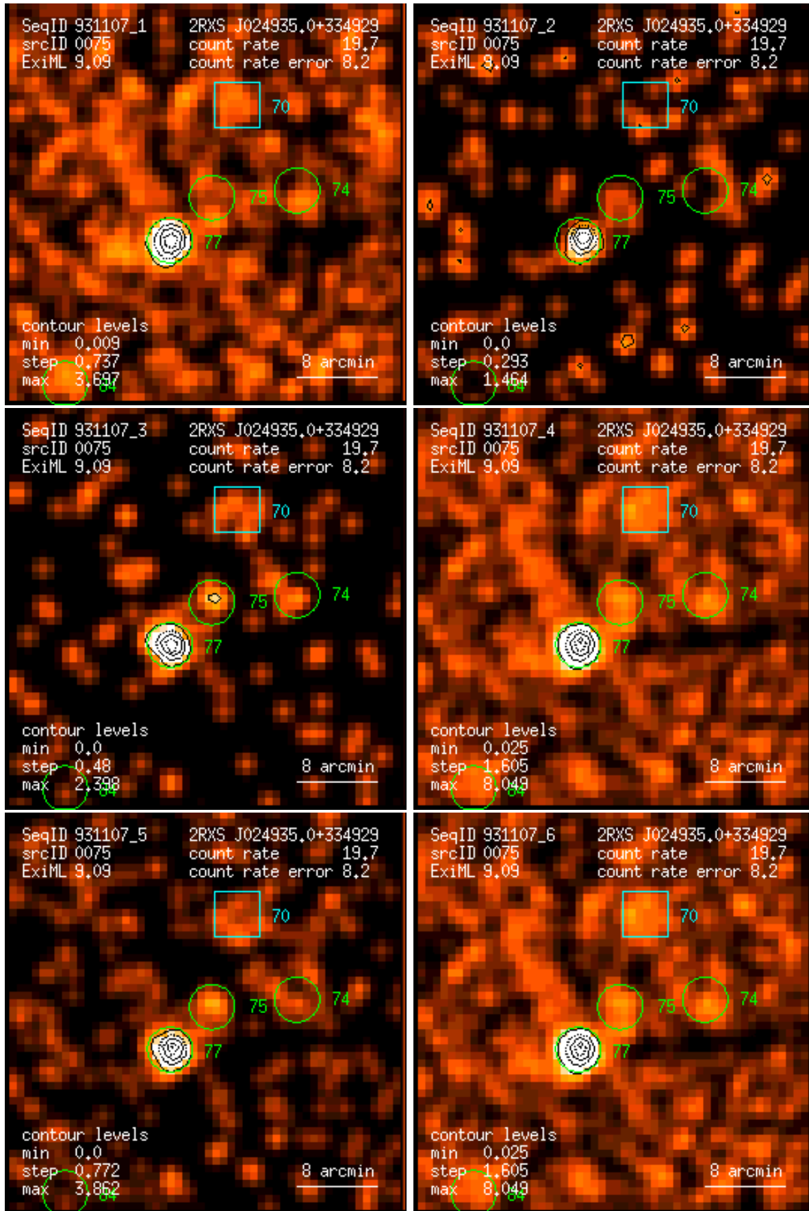
Figure 75: RASS 931107: detection 0075: band rate images, Gaussian filter: (1) PSPC channels 11 – 41, (2) 52 – 90, (3) 91 – 201, (4) 11 – 235, (5) 52 – 201, (6) 11 – 201. Broad band rates in counts/ks. Band rate contour levels in counts/ks/arcmin 2 .
