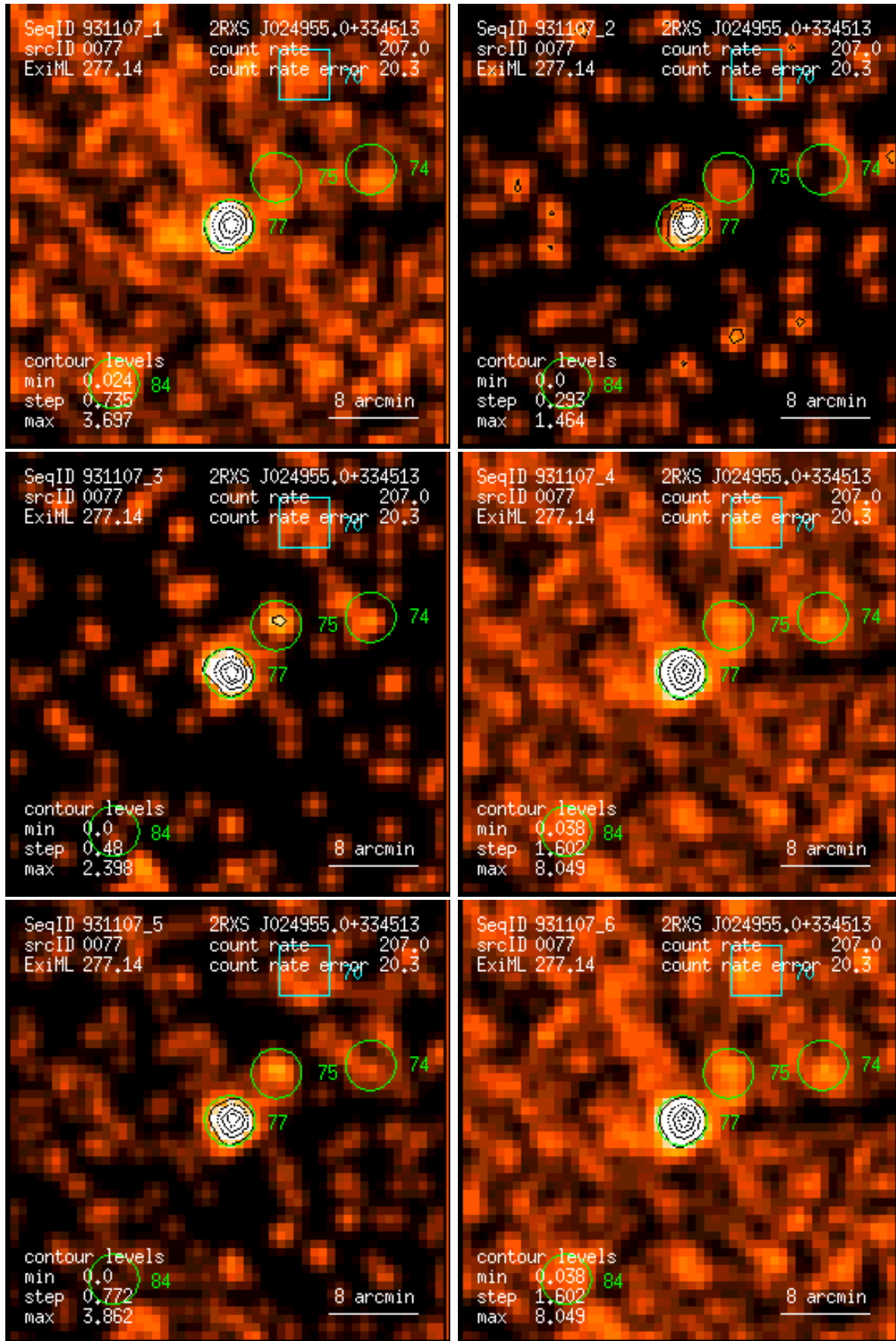
Figure 77: RASS 931107: detection 0077: band rate images, Gaussian filter: (1) PSPC channels 11 – 41, (2) 52 – 90, (3) 91 – 201, (4) 11 – 235, (5) 52 – 201, (6) 11 – 201. Broad band rates in counts/ks. Band rate contour levels in counts/ks/arcmin 2 .
