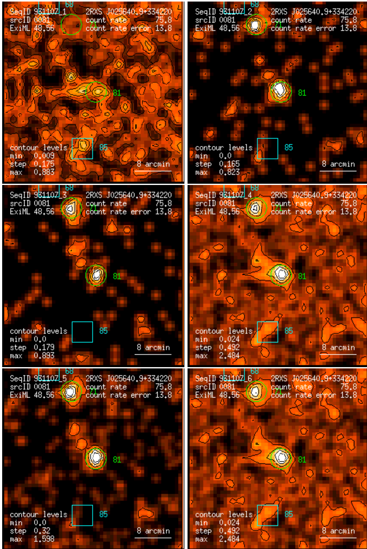
Figure 81: RASS 931107: detection 0081: band rate images, Gaussian filter: (1) PSPC channels 11 – 41, (2) 52 – 90, (3) 91 – 201, (4) 11 – 235, (5) 52 – 201, (6) 11 – 201. Broad band rates in counts/ks. Band rate contour levels in counts/ks/arcmin 2 .
