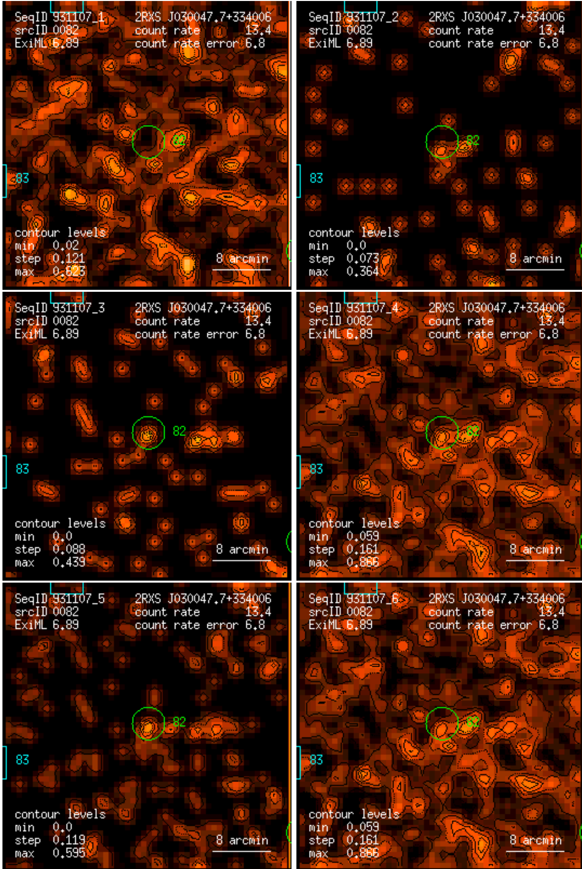
Figure 82: RASS 931107: detection 0082: band rate images, Gaussian filter: (1) PSPC channels 11 – 41, (2) 52 – 90, (3) 91 – 201, (4) 11 – 235, (5) 52 – 201, (6) 11 – 201. Broad band rates in counts/ks. Band rate contour levels in counts/ks/arcmin 2 .
