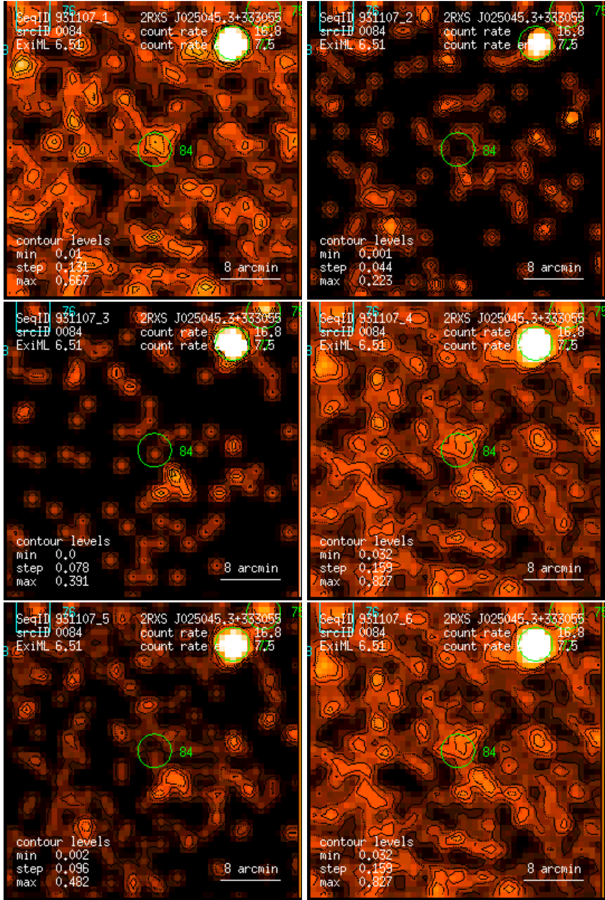
Figure 84: RASS 931107: detection 0084: band rate images, Gaussian filter: (1) PSPC channels 11 – 41, (2) 52 – 90, (3) 91 – 201, (4) 11 – 235, (5) 52 – 201, (6) 11 – 201. Broad band rates in counts/ks. Band rate contour levels in counts/ks/arcmin 2 .
