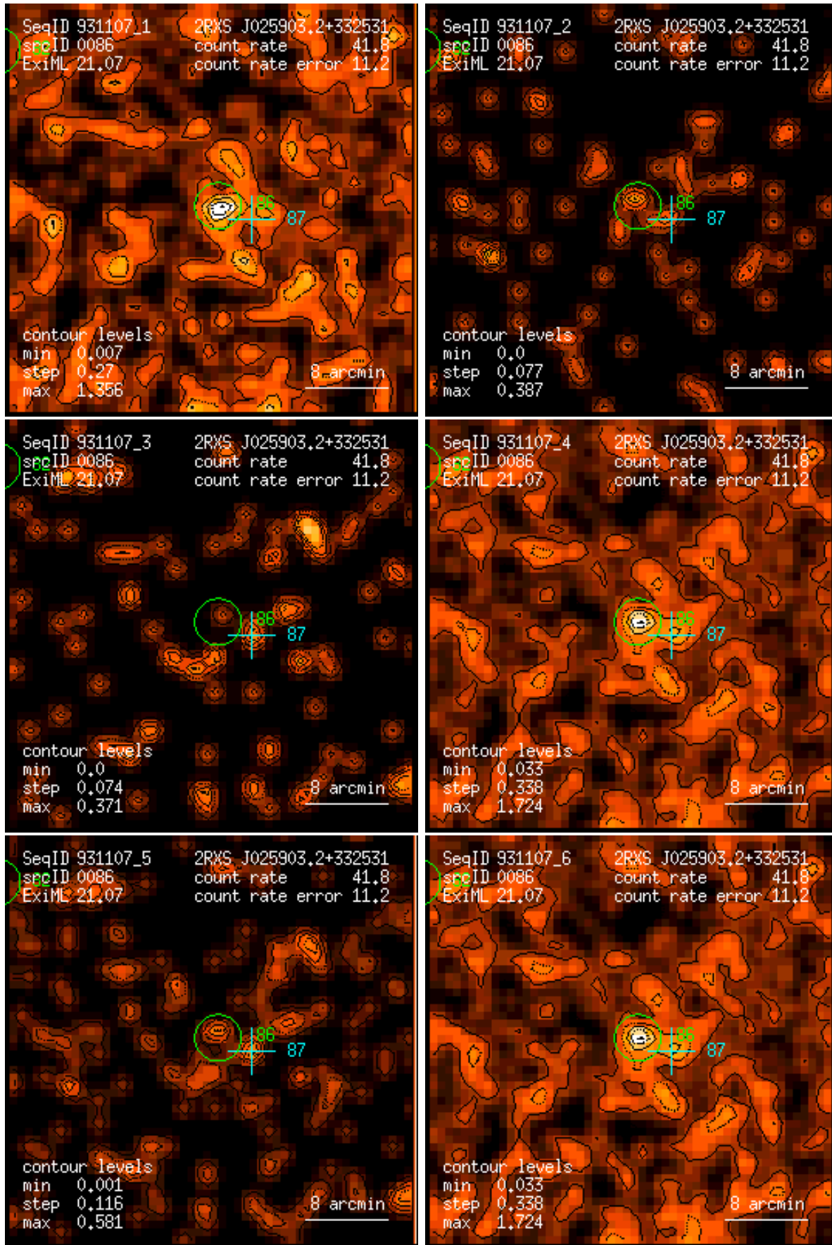
Figure 86: RASS 931107: detection 0086: band rate images, Gaussian filter: (1) PSPC channels 11 – 41, (2) 52 – 90, (3) 91 – 201, (4) 11 – 235, (5) 52 – 201, (6) 11 – 201. Broad band rates in counts/ks. Band rate contour levels in counts/ks/arcmin 2 .
