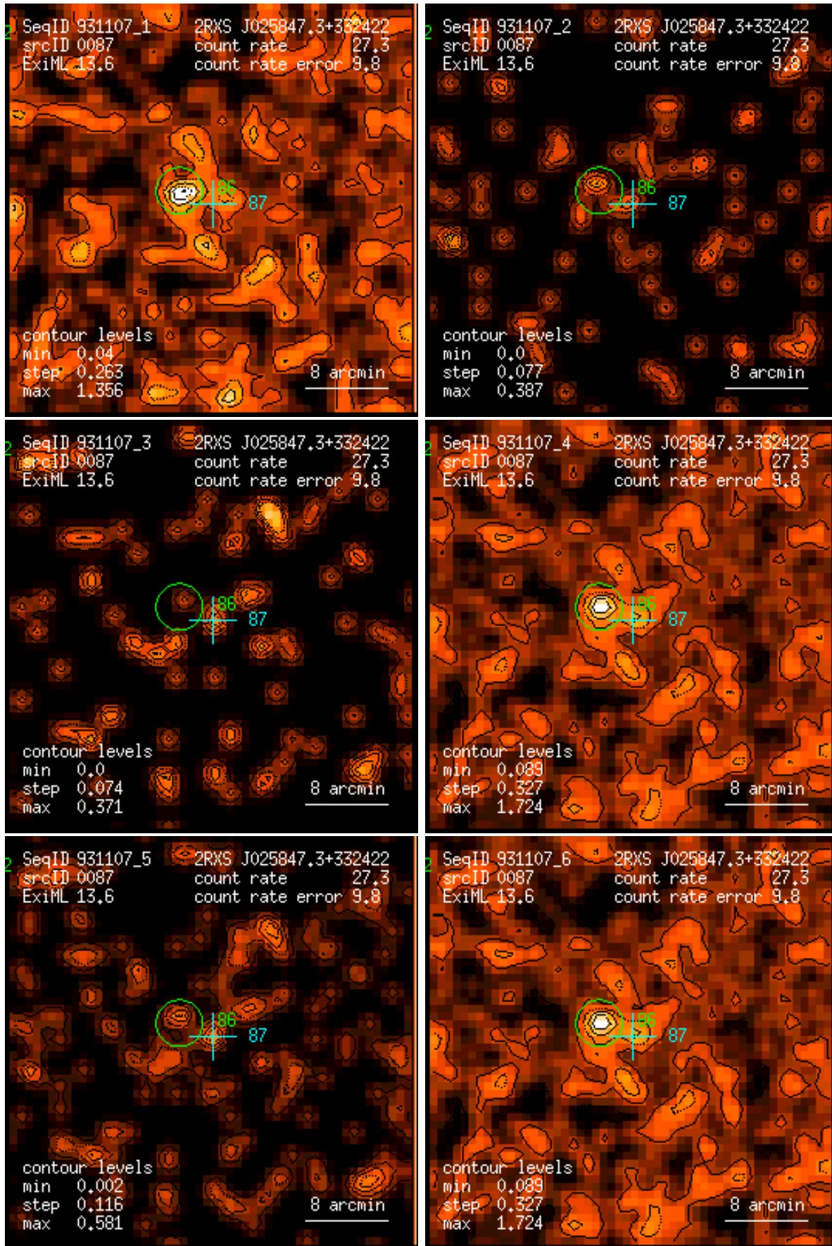
Figure 87: RASS 931107: detection 0087: band rate images, Gaussian filter: (1) PSPC channels 11 – 41, (2) 52 – 90, (3) 91 – 201, (4) 11 – 235, (5) 52 – 201, (6) 11 – 201. Broad band rates in counts/ks. Band rate contour levels in counts/ks/arcmin 2 .
