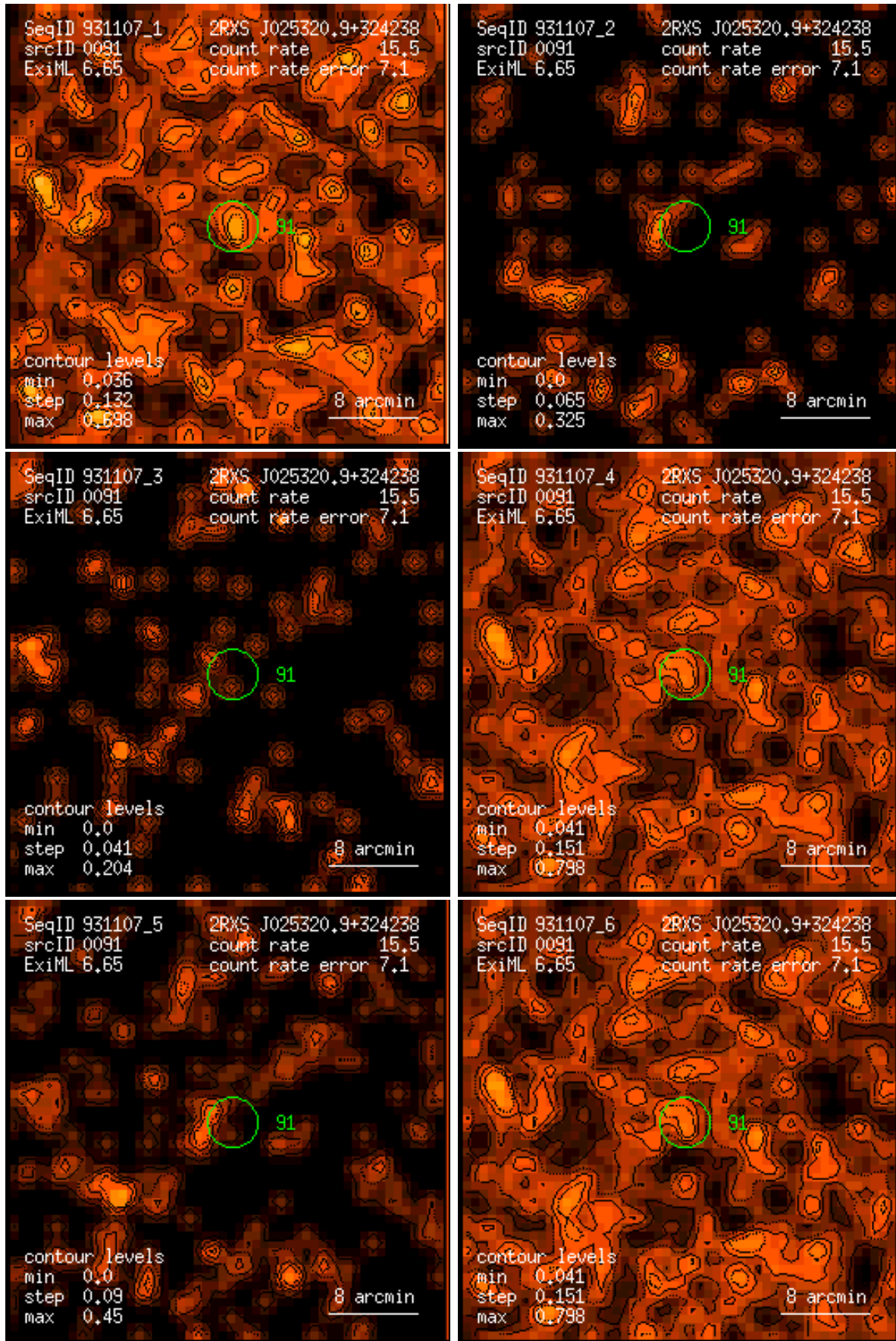
Figure 91: RASS 931107: detection 0091: band rate images, Gaussian filter: (1) PSPC channels 11 – 41, (2) 52 – 90, (3) 91 – 201, (4) 11 – 235, (5) 52 – 201, (6) 11 – 201. Broad band rates in counts/ks. Band rate contour levels in counts/ks/arcmin 2 .
