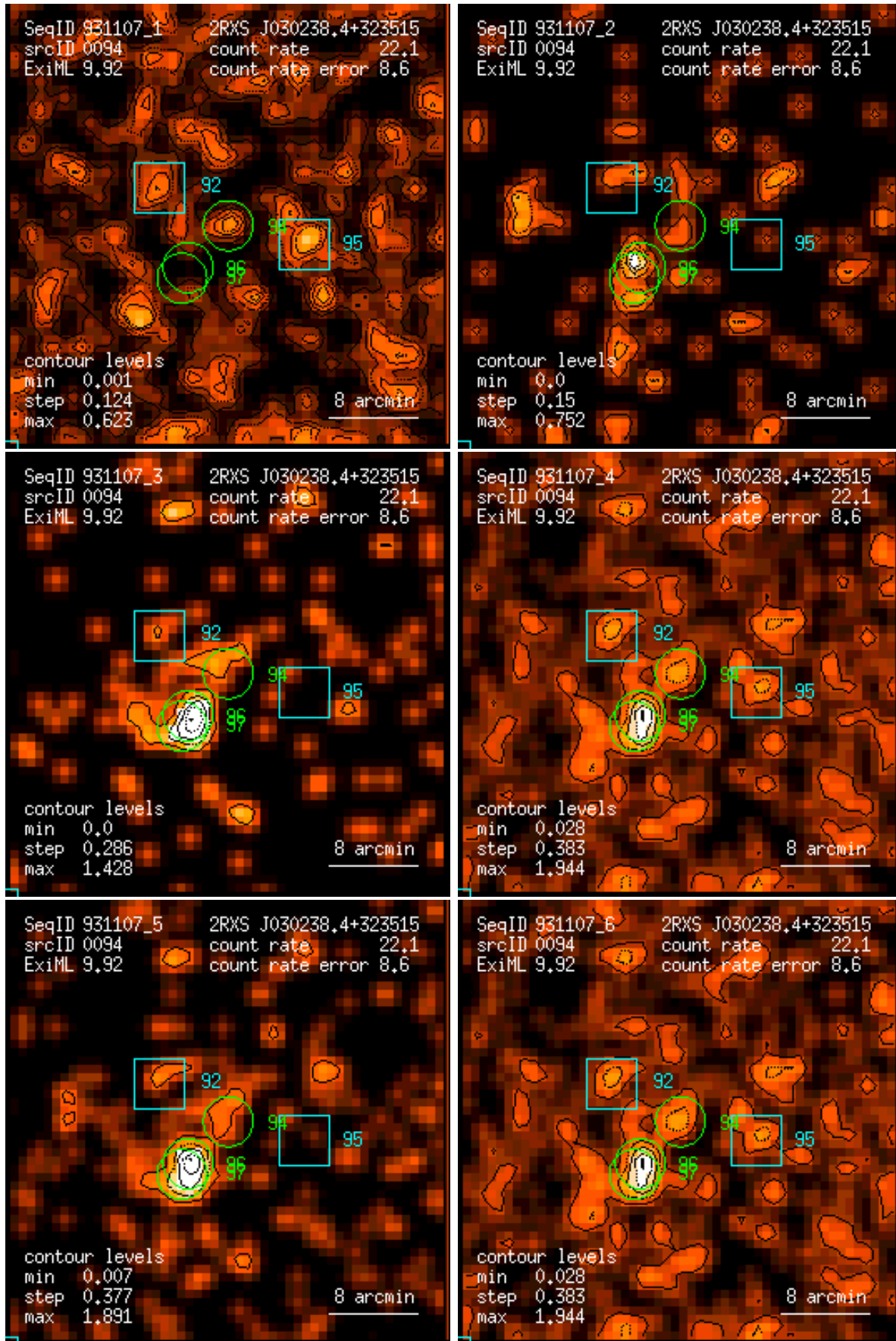
Figure 94: RASS 931107: detection 0094: band rate images, Gaussian filter: (1) PSPC channels 11 – 41, (2) 52 – 90, (3) 91 – 201, (4) 11 – 235, (5) 52 – 201, (6) 11 – 201. Broad band rates in counts/ks. Band rate contour levels in counts/ks/arcmin 2 .
