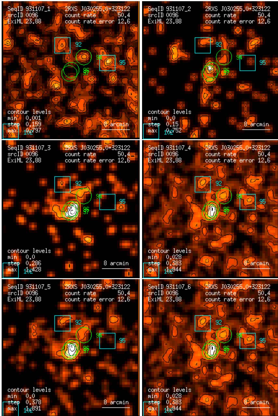
Figure 96: RASS 931107: detection 0096: band rate images, Gaussian filter: (1) PSPC channels 11 – 41, (2) 52 – 90, (3) 91 – 201, (4) 11 – 235, (5) 52 – 201, (6) 11 – 201. Broad band rates in counts/ks. Band rate contour levels in counts/ks/arcmin 2 .
