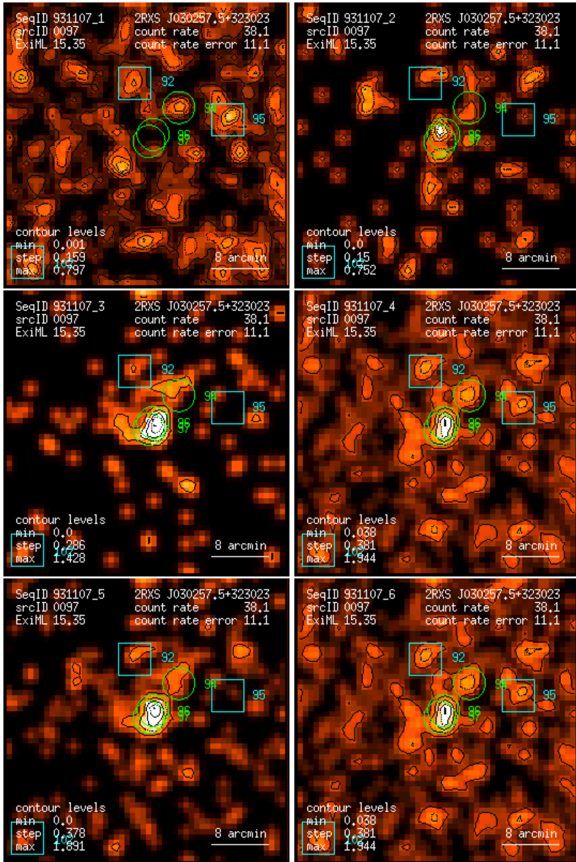
Figure 97: RASS 931107: detection 0097: band rate images, Gaussian filter: (1) PSPC channels 11 – 41, (2) 52 – 90, (3) 91 – 201, (4) 11 – 235, (5) 52 – 201, (6) 11 – 201. Broad band rates in counts/ks. Band rate contour levels in counts/ks/arcmin 2 .
