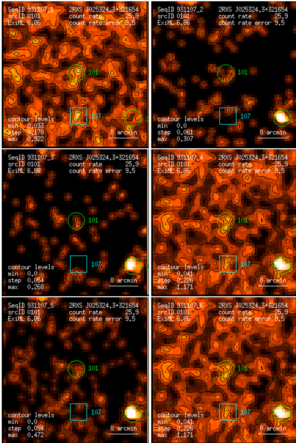
Figure 101: RASS 931107: detection 0101: band rate images, Gaussian filter: (1) PSPC channels 11 – 41, (2) 52 – 90, (3) 91 – 201, (4) 11 – 235, (5) 52 – 201, (6) 11 – 201. Broad band rates in counts/ks. Band rate contour levels in counts/ks/arcmin 2 .
