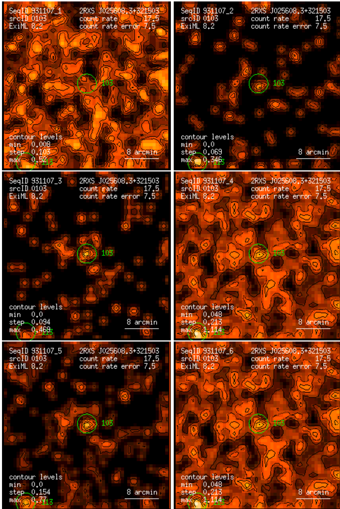
Figure 103: RASS 931107: detection 0103: band rate images, Gaussian filter: (1) PSPC channels 11 – 41, (2) 52 – 90, (3) 91 – 201, (4) 11 – 235, (5) 52 – 201, (6) 11 – 201. Broad band rates in counts/ks. Band rate contour levels in counts/ks/arcmin 2 .
