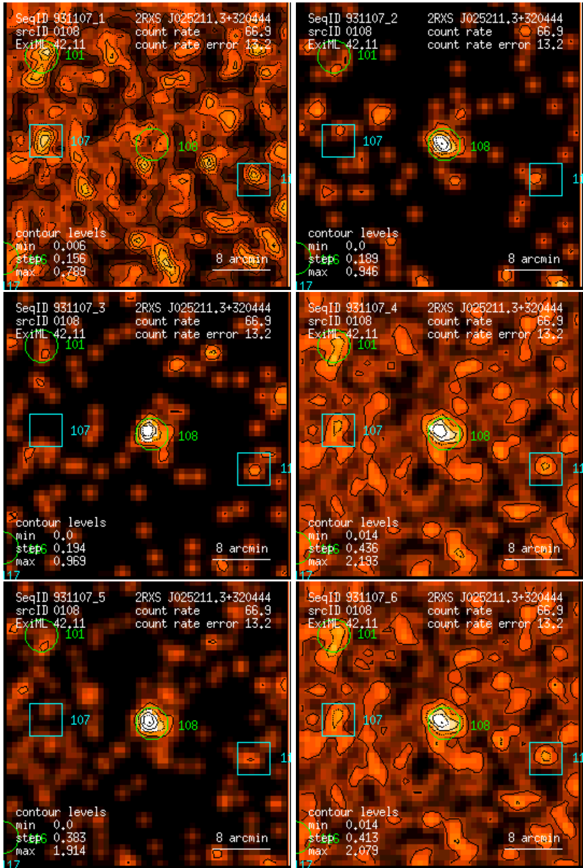
Figure 108: RASS 931107: detection 0108: band rate images, Gaussian filter: (1) PSPC channels 11 – 41, (2) 52 – 90, (3) 91 – 201, (4) 11 – 235, (5) 52 – 201, (6) 11 – 201. Broad band rates in counts/ks. Band rate contour levels in counts/ks/arcmin 2 .
