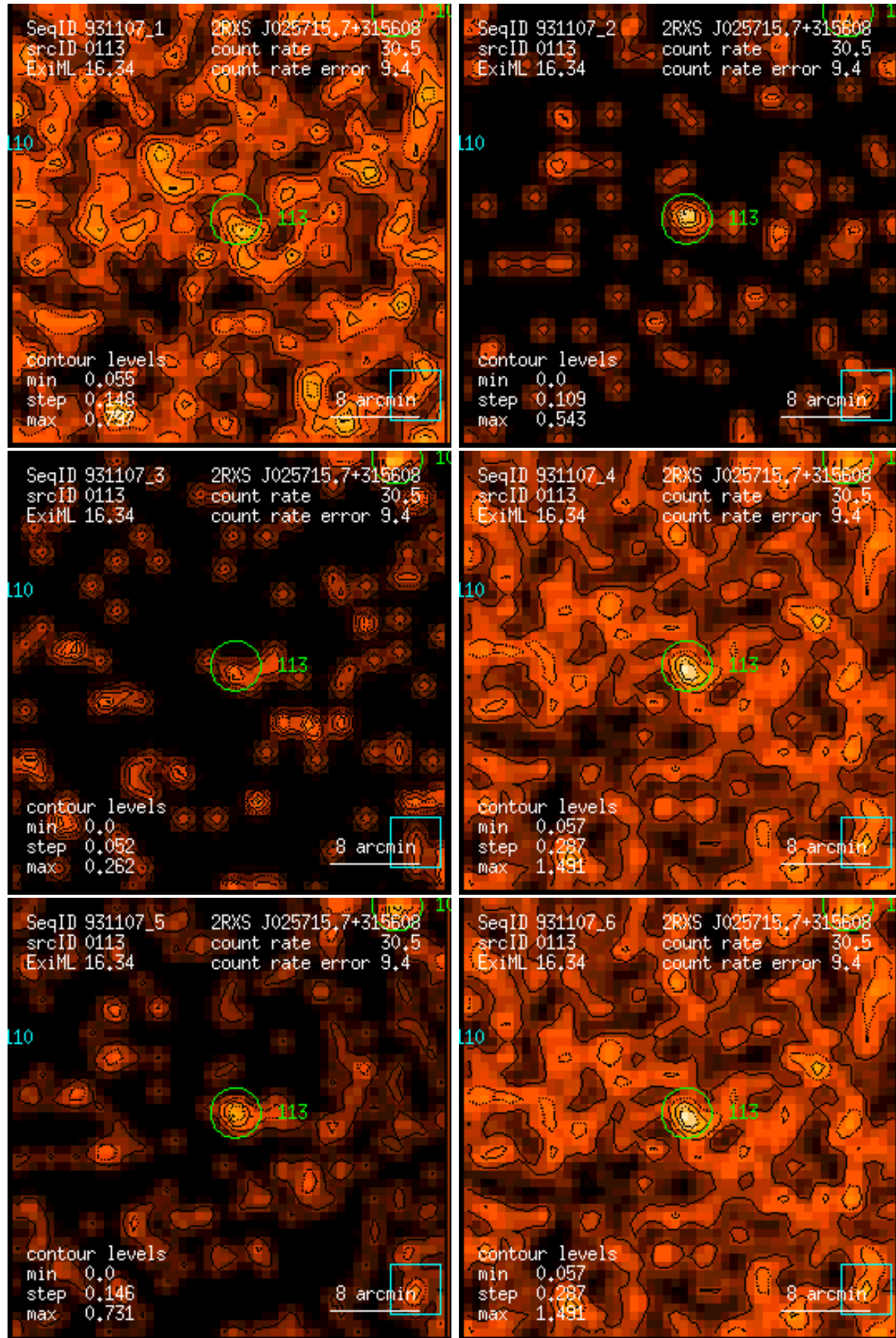
Figure 113: RASS 931107: detection 0113: band rate images, Gaussian filter: (1) PSPC channels 11 – 41, (2) 52 – 90, (3) 91 – 201, (4) 11 – 235, (5) 52 – 201, (6) 11 – 201. Broad band rates in counts/ks. Band rate contour levels in counts/ks/arcmin 2 .
