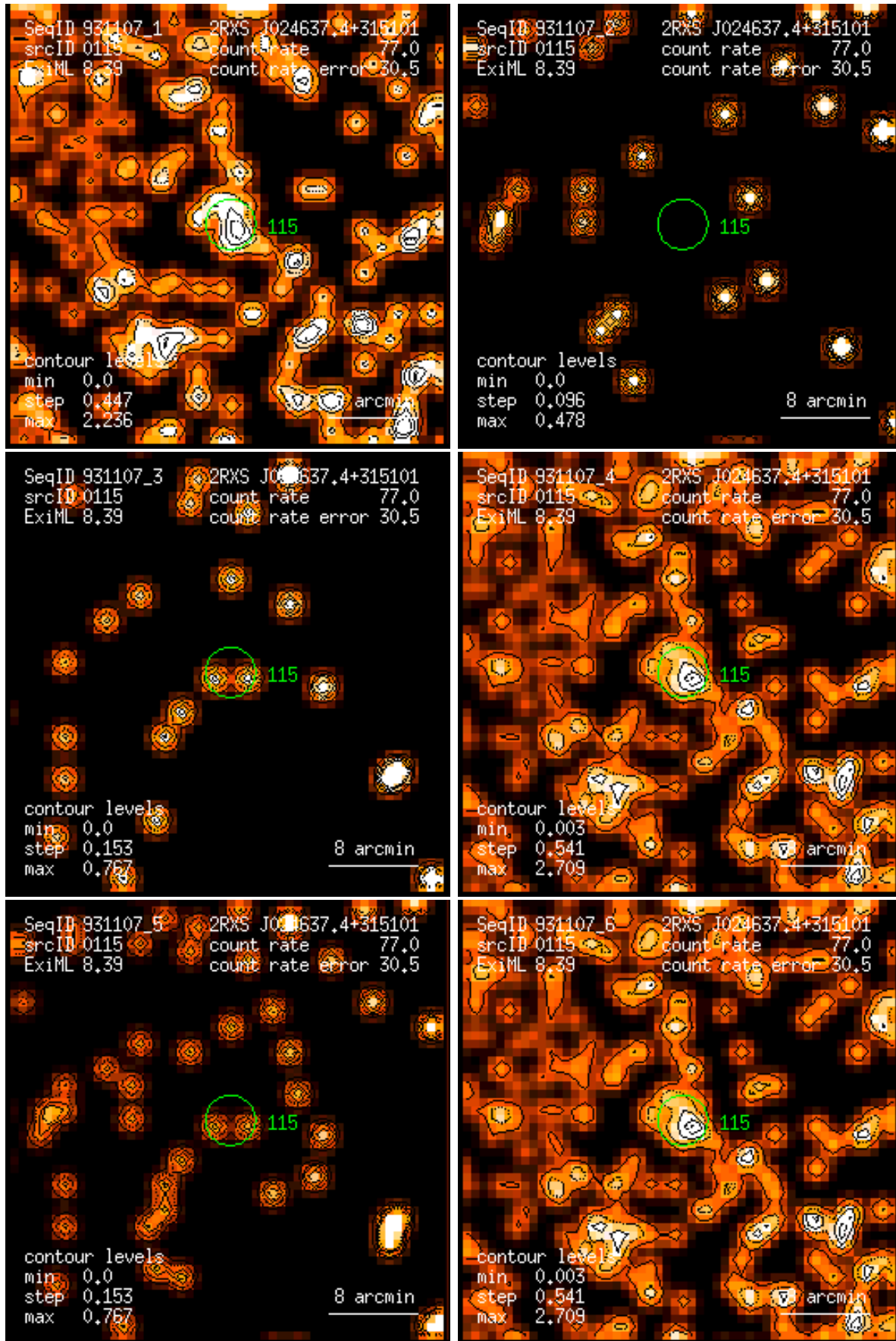
Figure 115: RASS 931107: detection 0115: band rate images, Gaussian filter: (1) PSPC channels 11 – 41, (2) 52 – 90, (3) 91 – 201, (4) 11 – 235, (5) 52 – 201, (6) 11 – 201. Broad band rates in counts/ks. Band rate contour levels in counts/ks/arcmin 2 .
