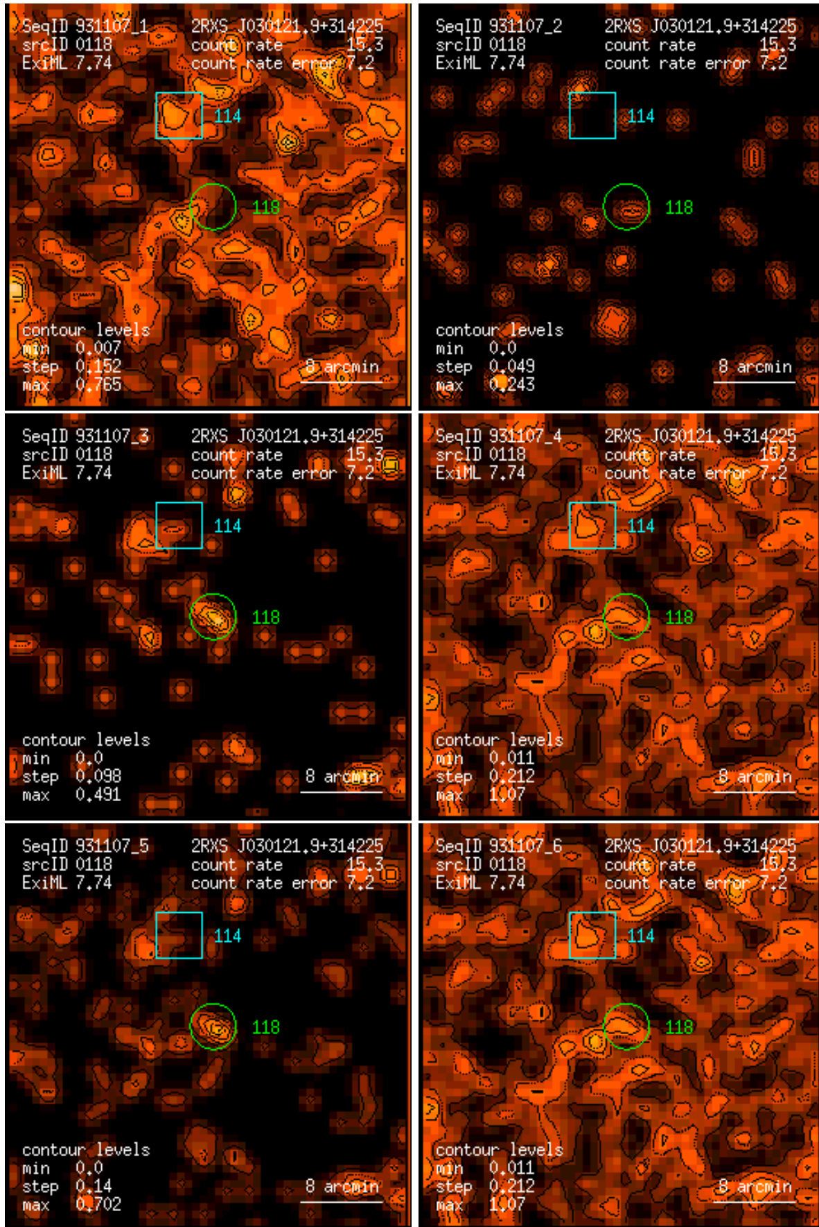
Figure 118: RASS 931107: detection 0118: band rate images, Gaussian filter: (1) PSPC channels 11 – 41, (2) 52 – 90, (3) 91 – 201, (4) 11 – 235, (5) 52 – 201, (6) 11 – 201. Broad band rates in counts/ks. Band rate contour levels in counts/ks/arcmin 2 .
