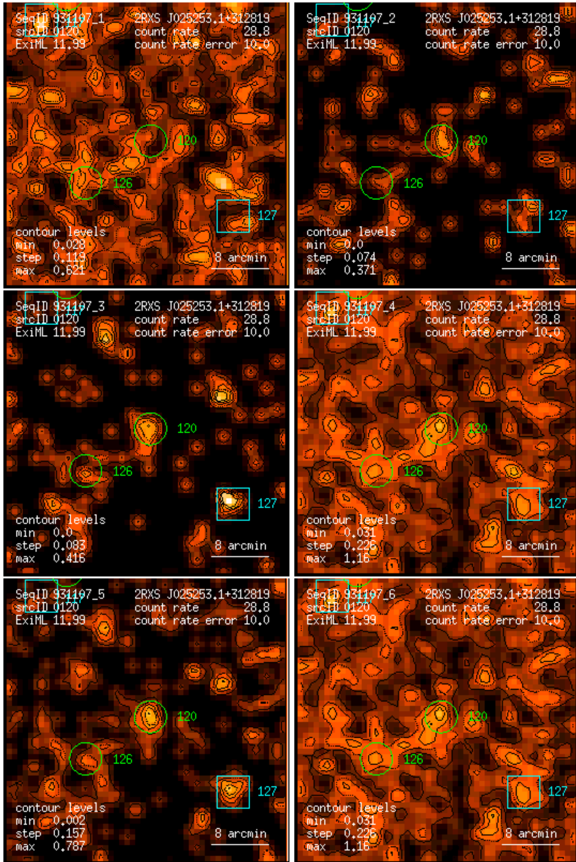
Figure 120: RASS 931107: detection 0120: band rate images, Gaussian filter: (1) PSPC channels 11 – 41, (2) 52 – 90, (3) 91 – 201, (4) 11 – 235, (5) 52 – 201, (6) 11 – 201. Broad band rates in counts/ks. Band rate contour levels in counts/ks/arcmin 2 .
