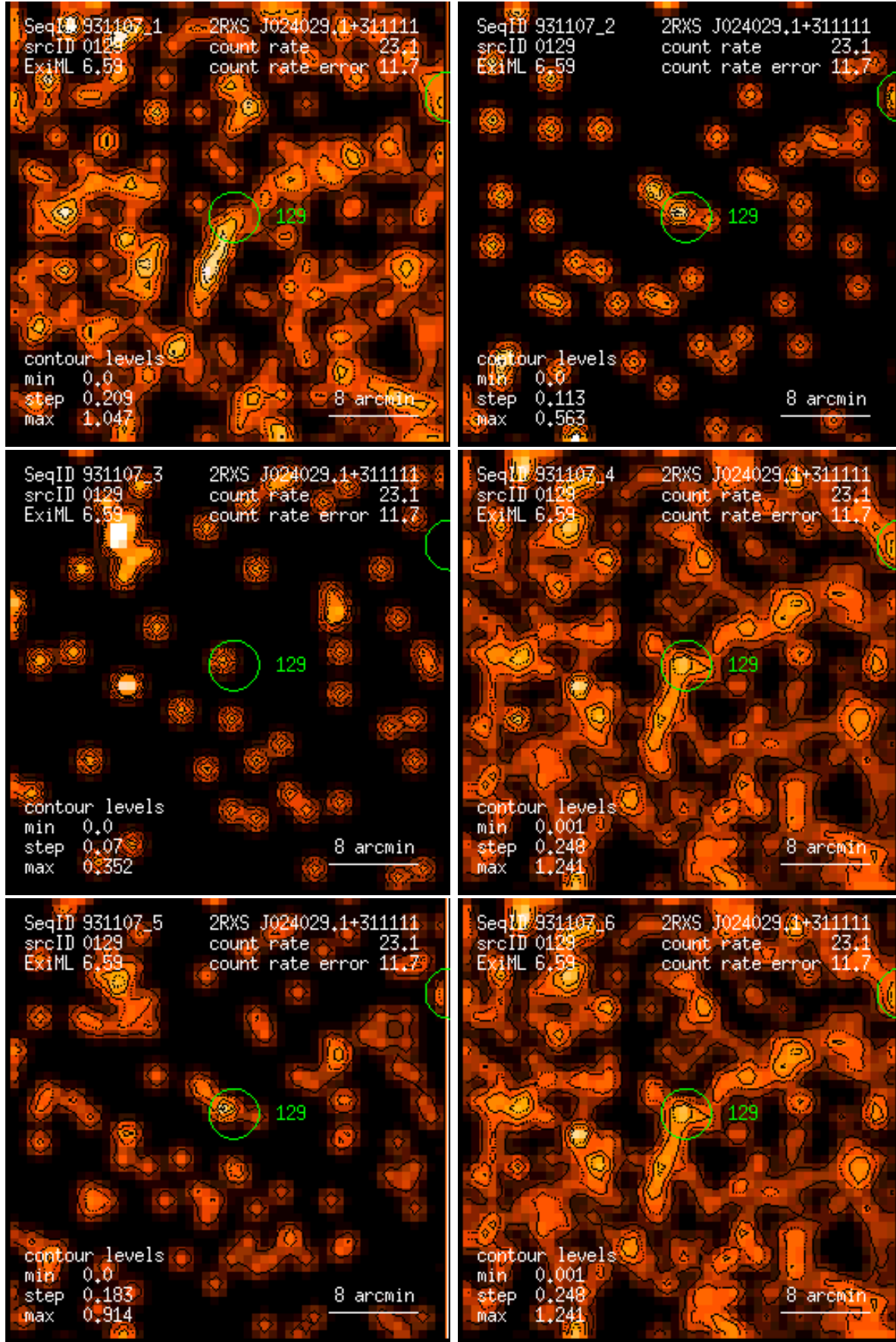
Figure 129: RASS 931107: detection 0129: band rate images, Gaussian filter: (1) PSPC channels 11 – 41, (2) 52 – 90, (3) 91 – 201, (4) 11 – 235, (5) 52 – 201, (6) 11 – 201. Broad band rates in counts/ks. Band rate contour levels in counts/ks/arcmin 2 .
