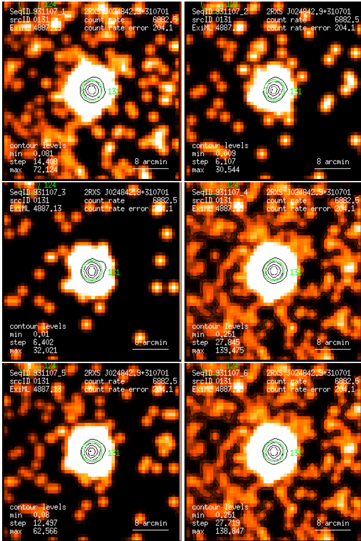
Figure 131: RASS 931107: detection 0131: band rate images, Gaussian filter: (1) PSPC channels 11 – 41, (2) 52 – 90, (3) 91 – 201, (4) 11 – 235, (5) 52 – 201, (6) 11 – 201. Broad band rates in counts/ks. Band rate contour levels in counts/ks/arcmin 2 .
