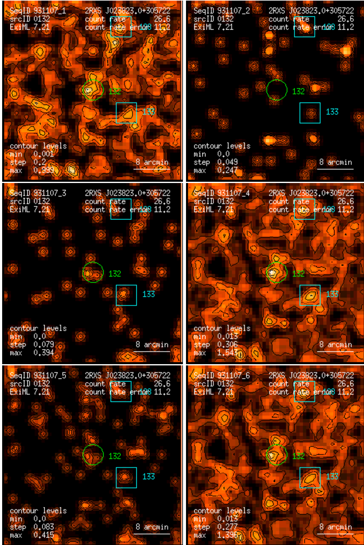
Figure 132: RASS 931107: detection 0132: band rate images, Gaussian filter: (1) PSPC channels 11 – 41, (2) 52 – 90, (3) 91 – 201, (4) 11 – 235, (5) 52 – 201, (6) 11 – 201. Broad band rates in counts/ks. Band rate contour levels in counts/ks/arcmin 2 .
