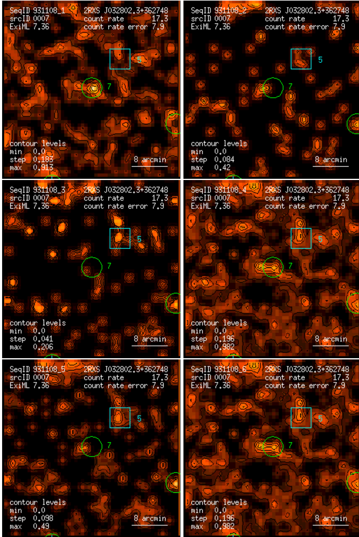
Figure 7: RASS 931108: detection 0007: band rate images, Gaussian filter: (1) PSPC channels 11 – 41, (2) 52 – 90, (3) 91 – 201, (4) 11 – 235, (5) 52 – 201, (6) 11 – 201. Broad band rates in counts/ks. Band rate contour levels in counts/ks/arcmin 2 .
