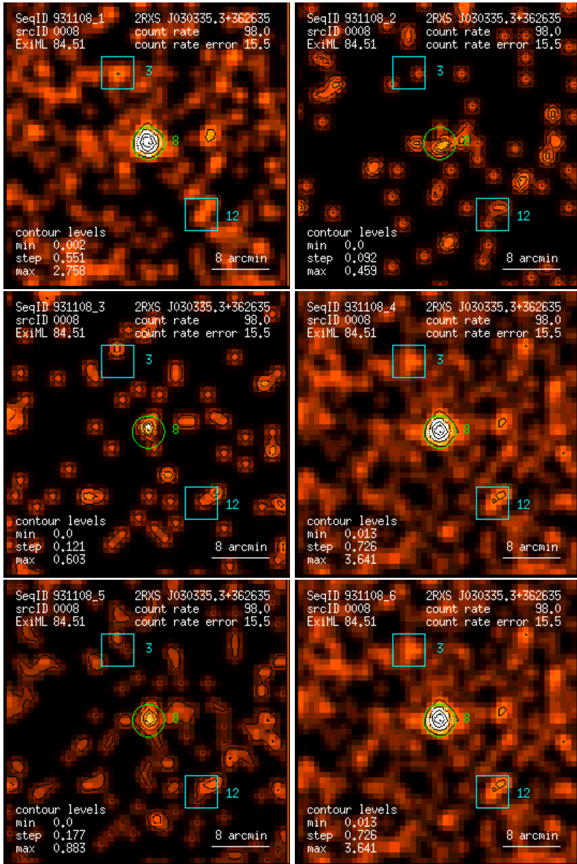
Figure 8: RASS 931108: detection 0008: band rate images, Gaussian filter: (1) PSPC channels 11 – 41, (2) 52 – 90, (3) 91 – 201, (4) 11 – 235, (5) 52 – 201, (6) 11 – 201. Broad band rates in counts/ks. Band rate contour levels in counts/ks/arcmin 2 .
