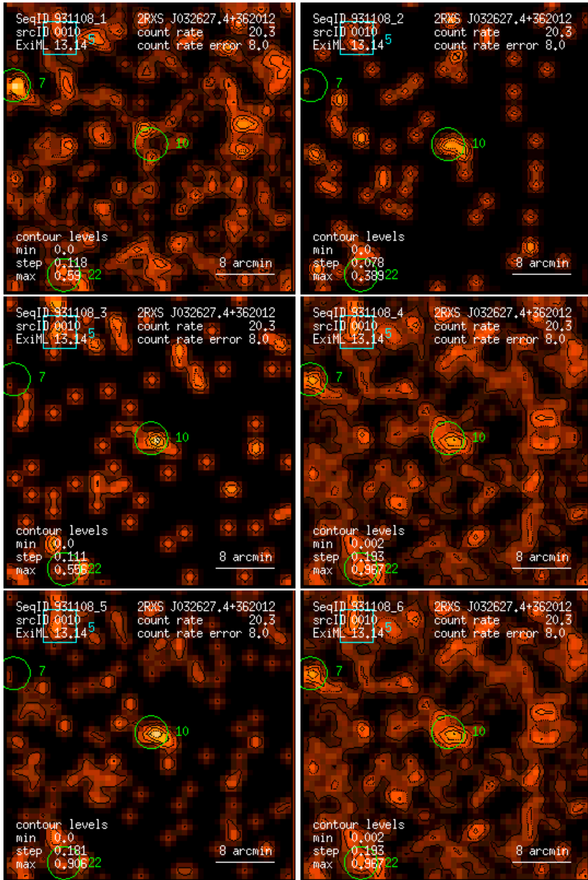
Figure 10: RASS 931108: detection 0010: band rate images, Gaussian filter: (1) PSPC channels 11 – 41, (2) 52 – 90, (3) 91 – 201, (4) 11 – 235, (5) 52 – 201, (6) 11 – 201. Broad band rates in counts/ks. Band rate contour levels in counts/ks/arcmin 2 .
