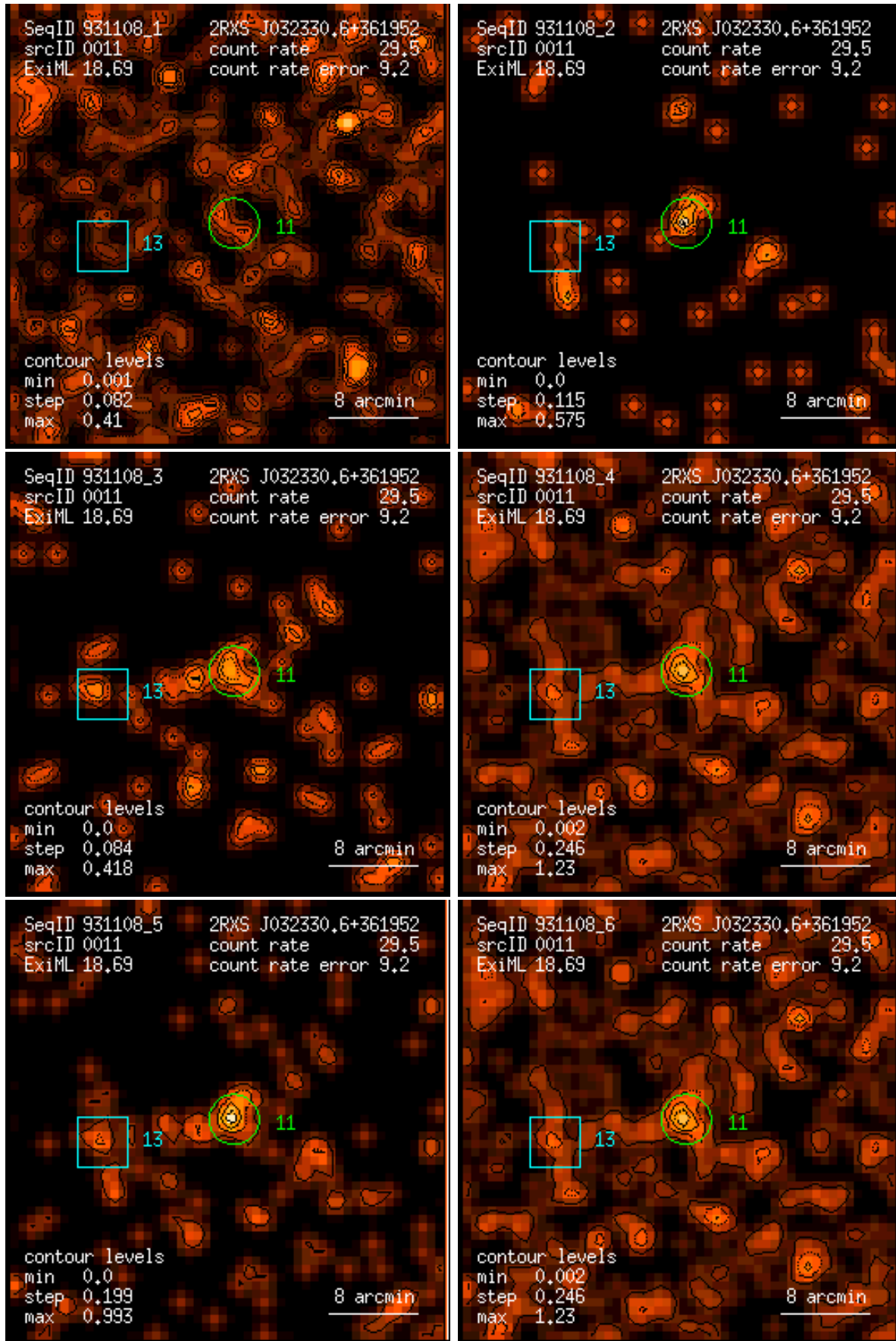
Figure 11: RASS 931108: detection 0011: band rate images, Gaussian filter: (1) PSPC channels 11 – 41, (2) 52 – 90, (3) 91 – 201, (4) 11 – 235, (5) 52 – 201, (6) 11 – 201. Broad band rates in counts/ks. Band rate contour levels in counts/ks/arcmin 2 .
