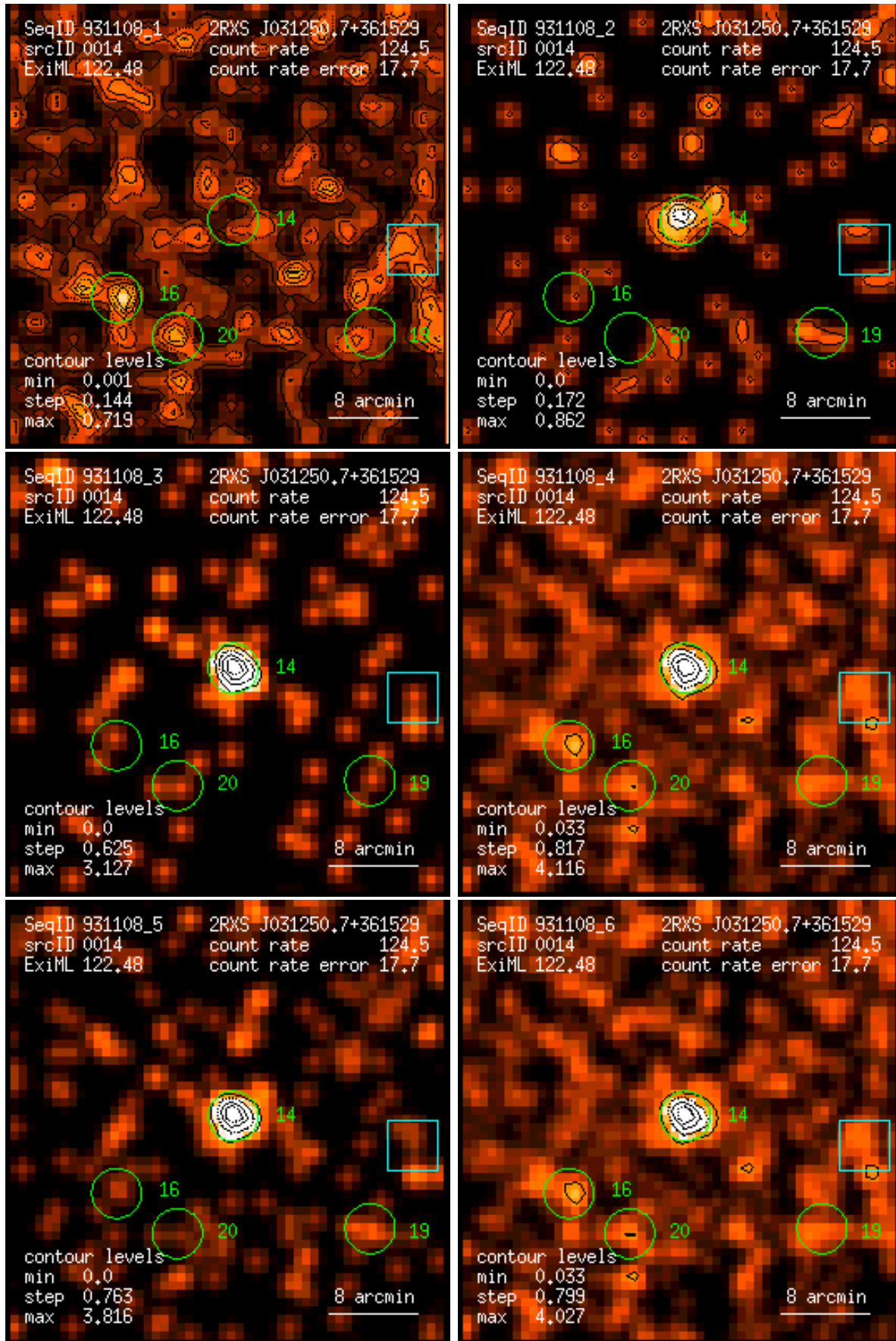
Figure 14: RASS 931108: detection 0014: band rate images, Gaussian filter: (1) PSPC channels 11 – 41, (2) 52 – 90, (3) 91 – 201, (4) 11 – 235, (5) 52 – 201, (6) 11 – 201. Broad band rates in counts/ks. Band rate contour levels in counts/ks/arcmin 2 .
