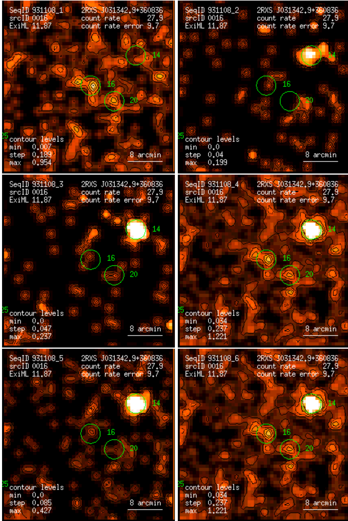
Figure 16: RASS 931108: detection 0016: band rate images, Gaussian filter: (1) PSPC channels 11 – 41, (2) 52 – 90, (3) 91 – 201, (4) 11 – 235, (5) 52 – 201, (6) 11 – 201. Broad band rates in counts/ks. Band rate contour levels in counts/ks/arcmin 2 .
