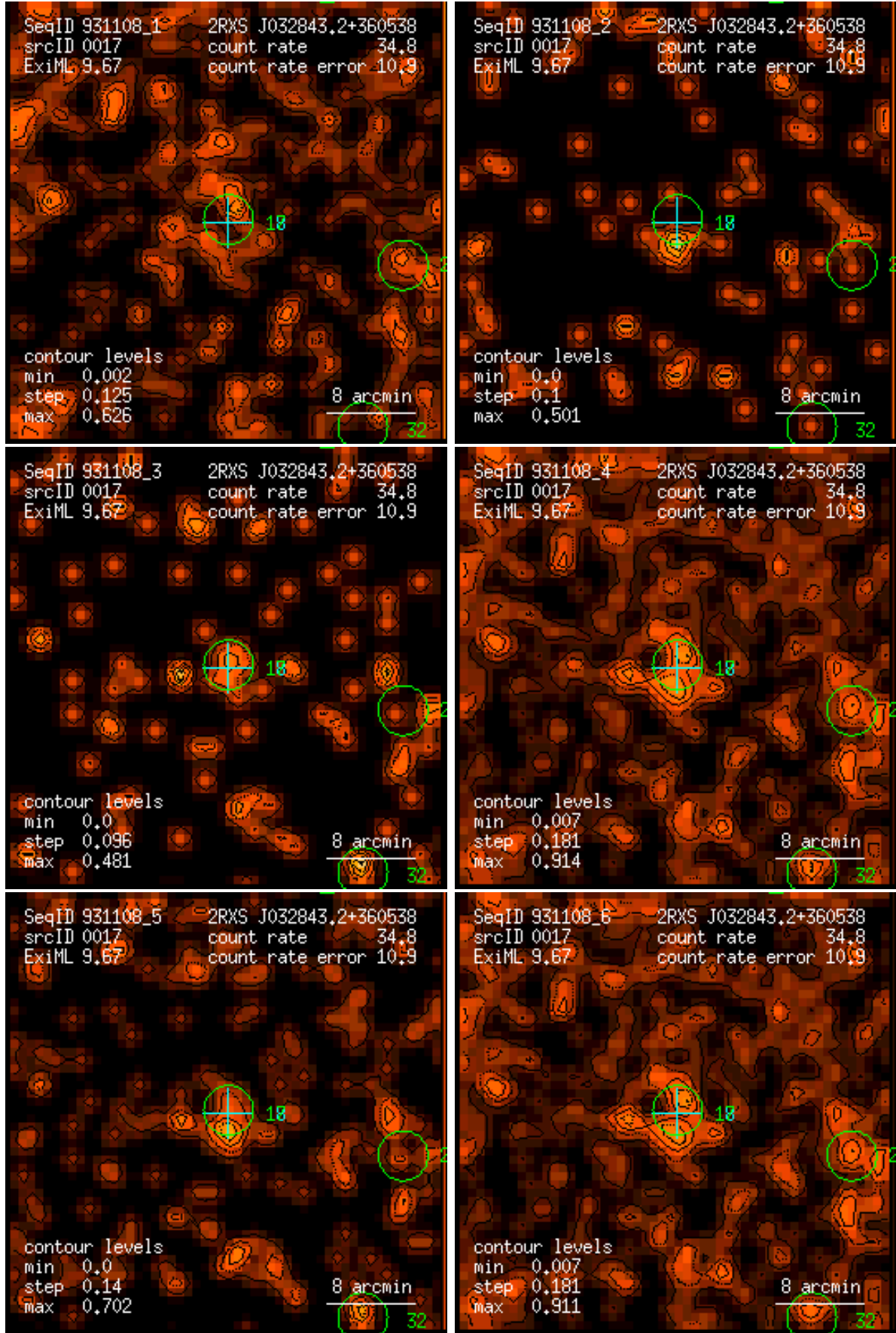
Figure 17: RASS 931108: detection 0017: band rate images, Gaussian filter: (1) PSPC channels 11 – 41, (2) 52 – 90, (3) 91 – 201, (4) 11 – 235, (5) 52 – 201, (6) 11 – 201. Broad band rates in counts/ks. Band rate contour levels in counts/ks/arcmin 2 .
